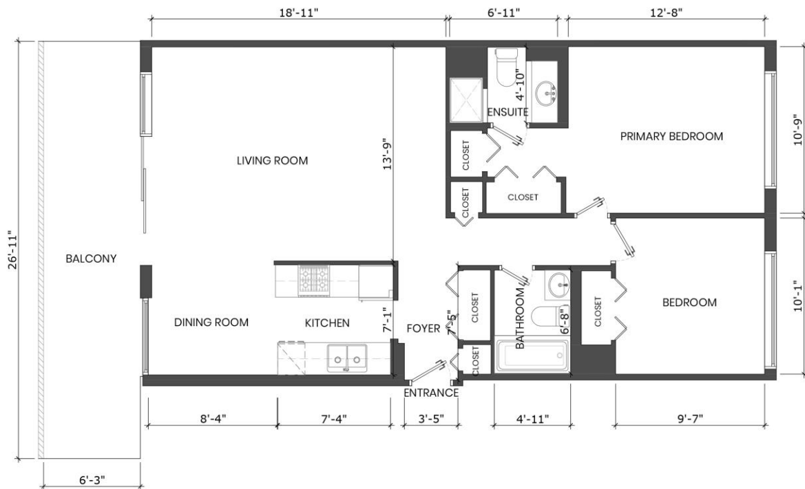
MAIN FLOOR PLAN Ceiling Height: 8'-0"
