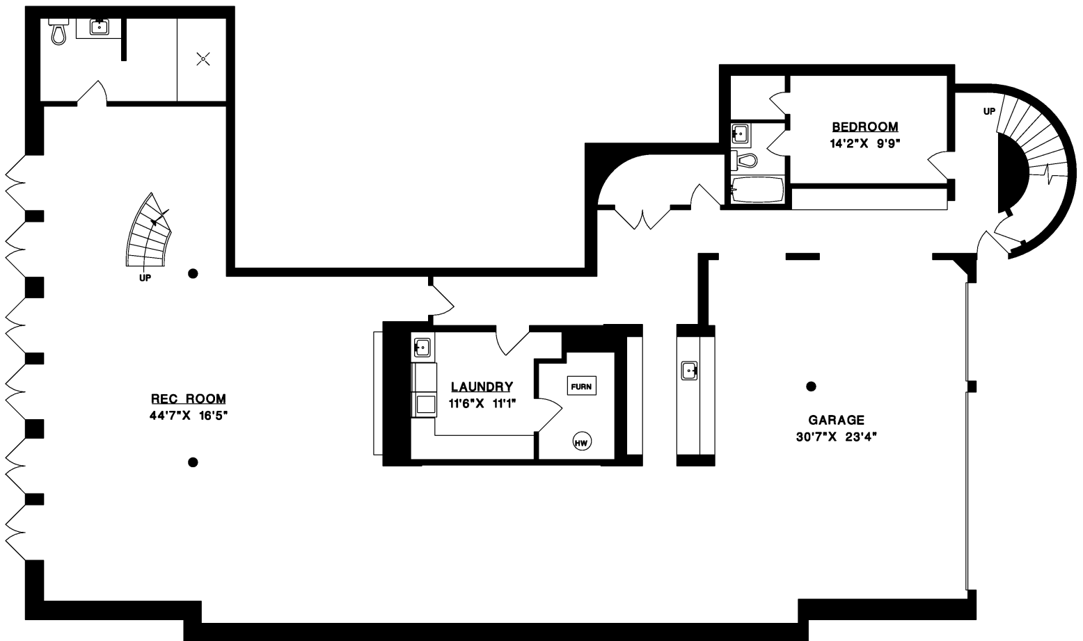
LOWER FLOOR
