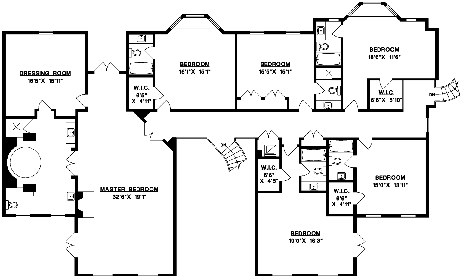
UPPER FLOOR
