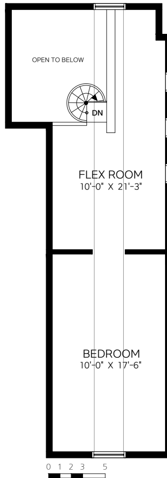
Upper Floor Ceiling Height: 5'-6"
