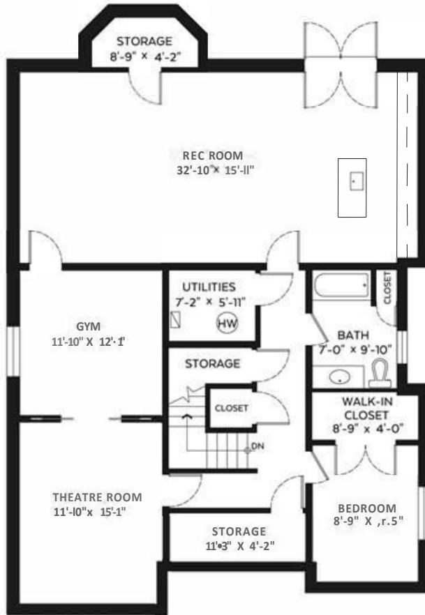
Lower Floor Plan Floor Area: 1,574 sq.ft.
