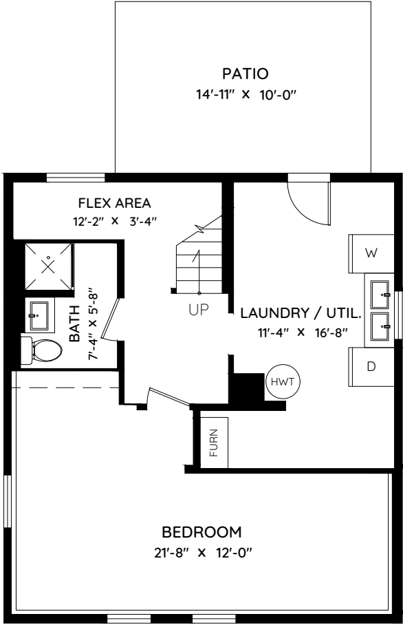
LOWER FLOOR 608 SQ.FT. CH: 6'-5"
