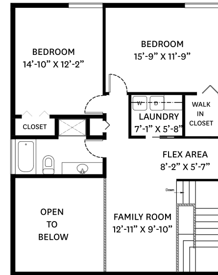
UPPER FLOOR PLAN Ceiling Height: 8'-0"
