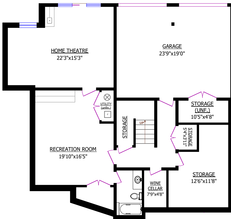
LOWER LEVEL
