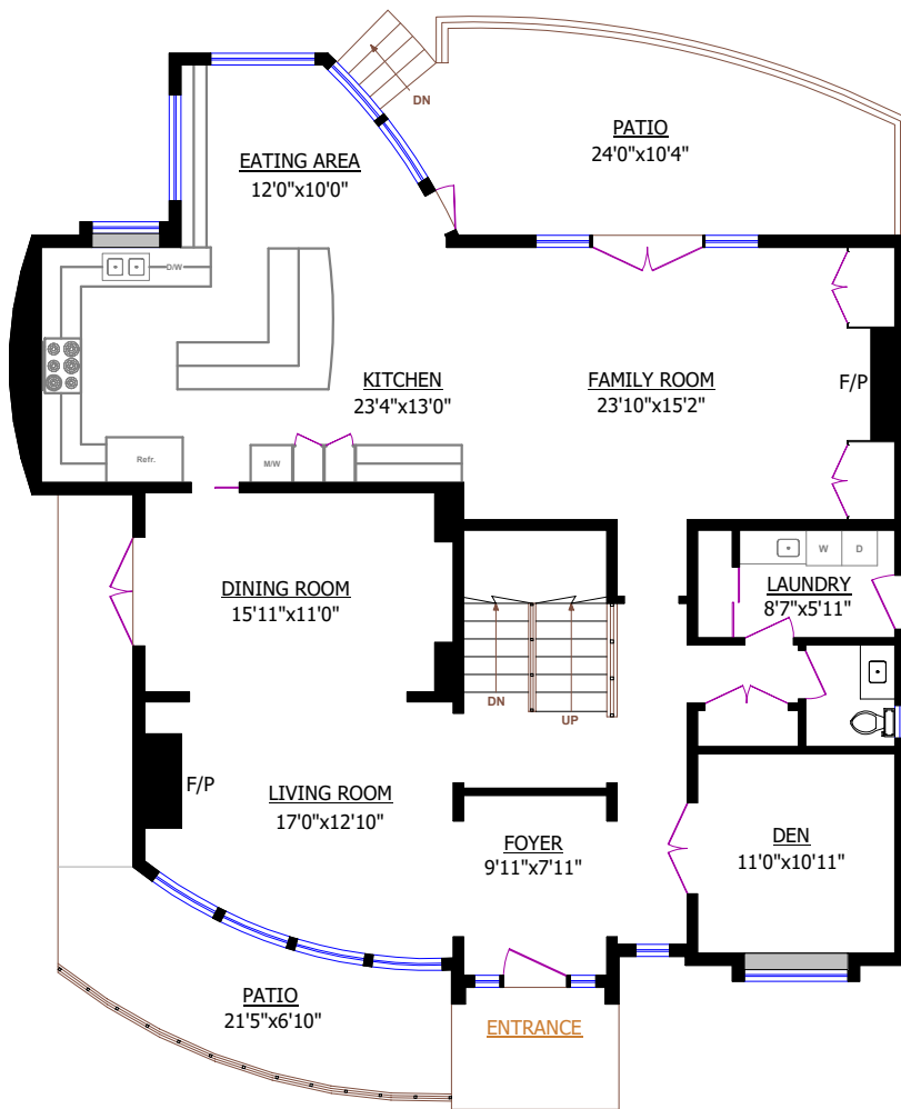
MAIN FLOOR
