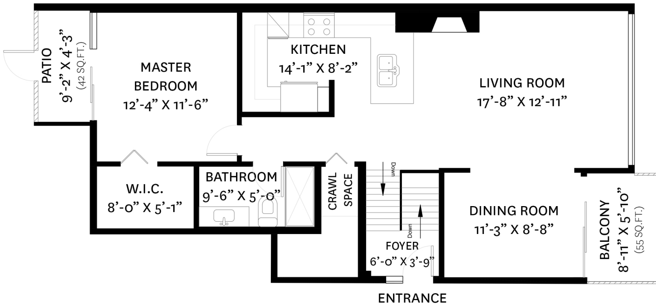
MAIN FLOOR PLAN Ceiling Height: 7'-11"
