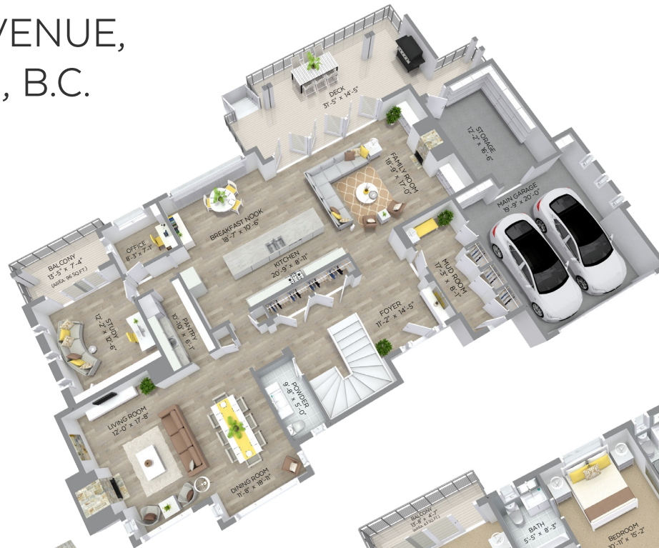
Main Floor Plan Floor Area: 2,238 sq.ft. Ceiling Height: 8'-11"
