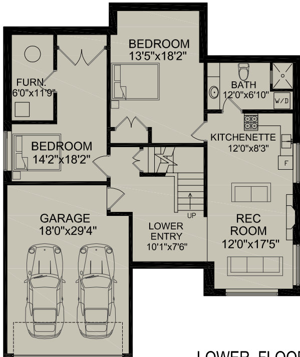
LOWER FLOOR
