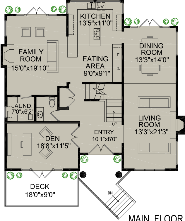
MAIN FLOOR
