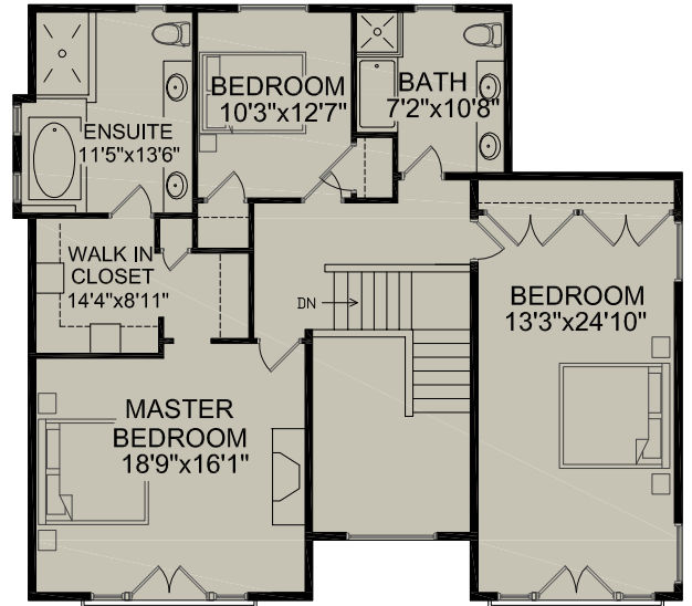
UPPER FLOOR
