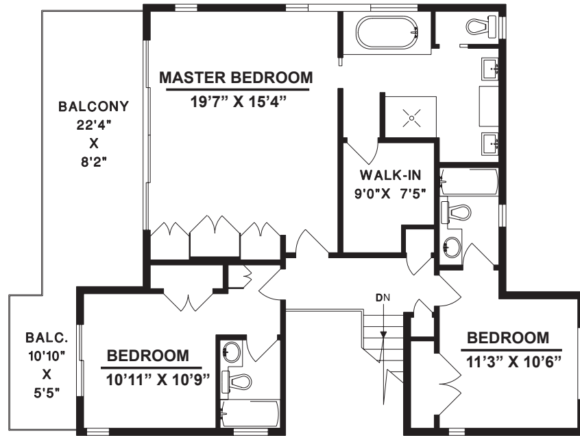
UPPER FLOOR
