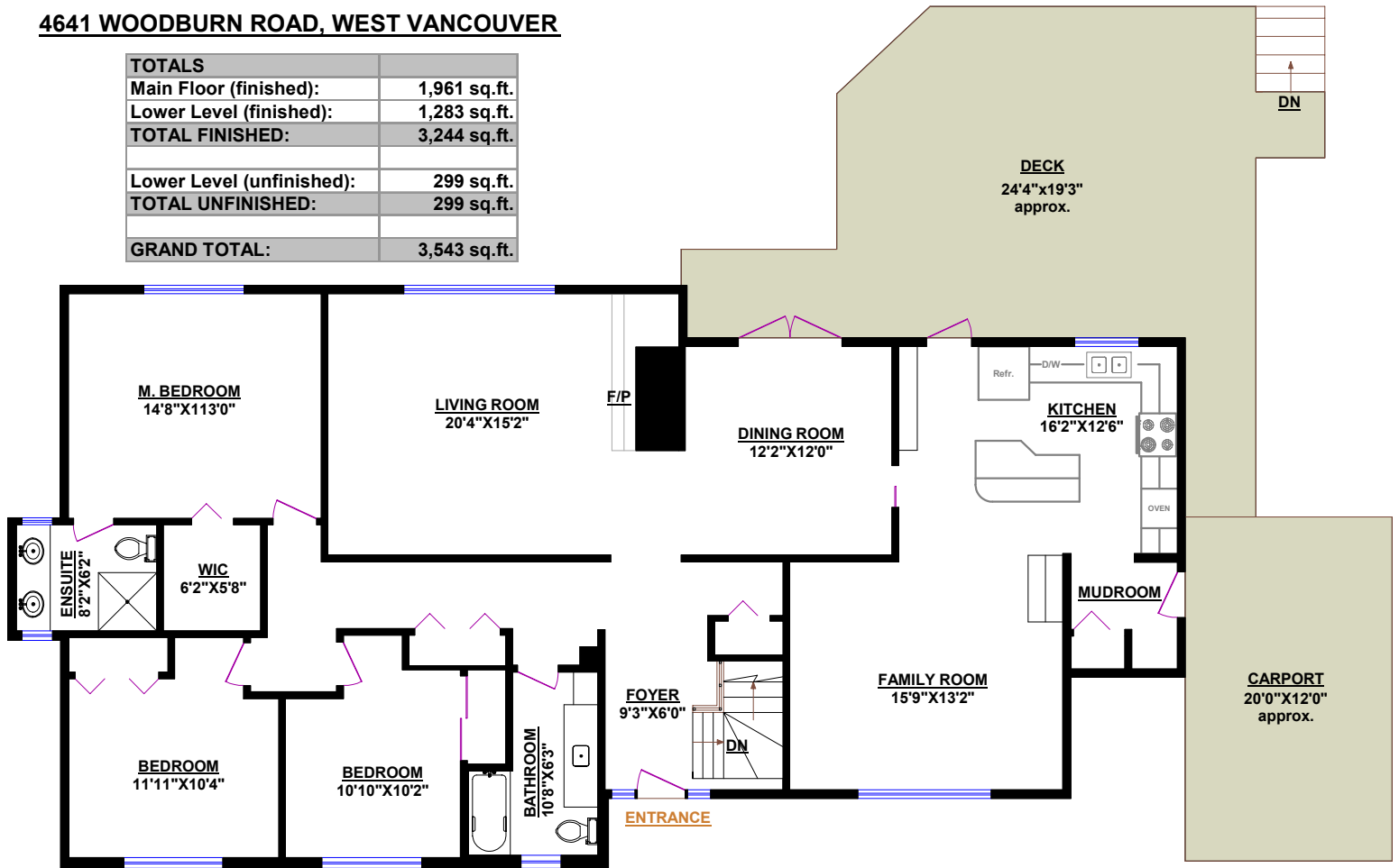
MAIN FLOOR
