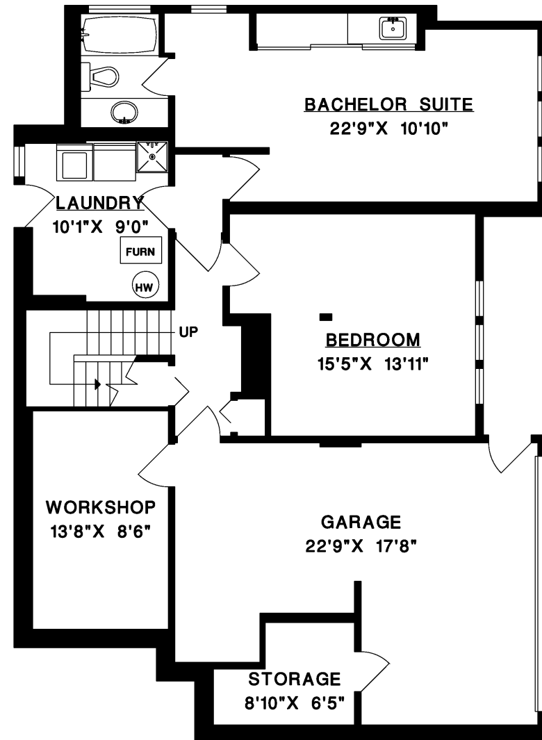
LOWER FLOOR
