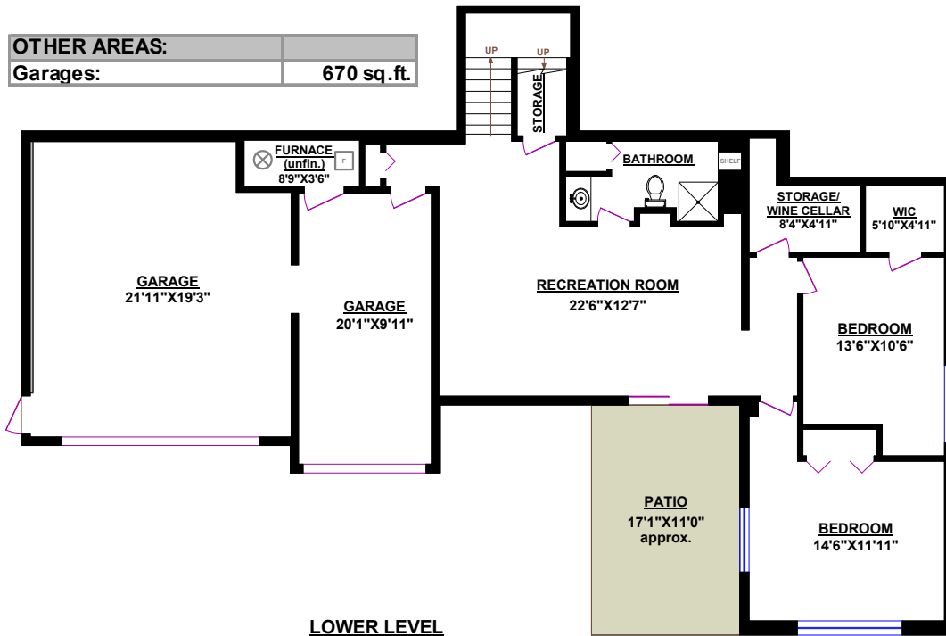
LOWER LEVEL
