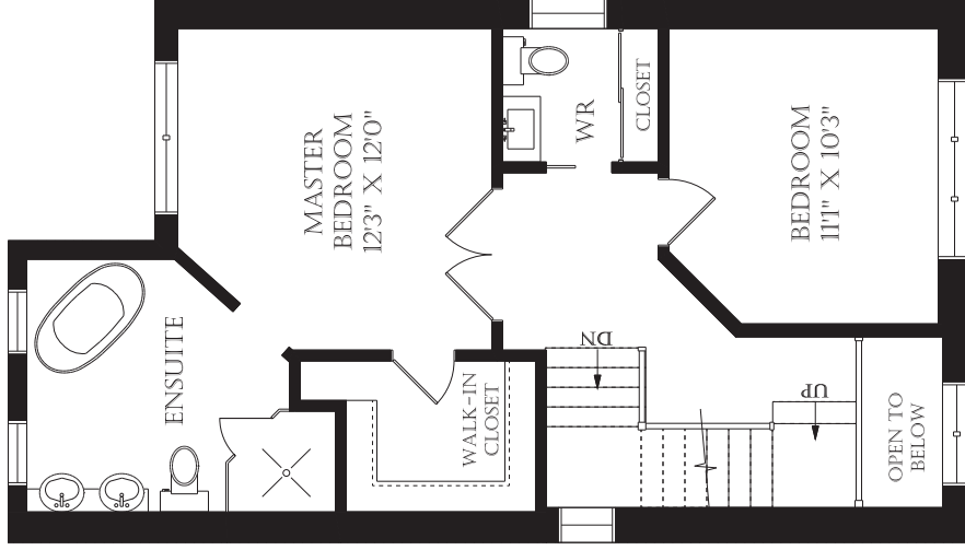
SECOND FLOOR 709 SQUARE FEET AREA INCLUDES OPEN TO BELOW
