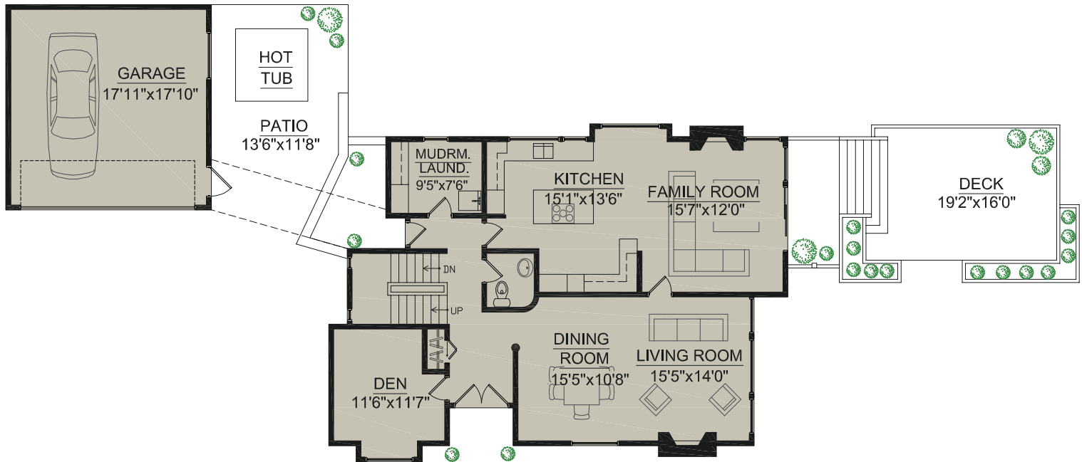
MAIN FLOOR
