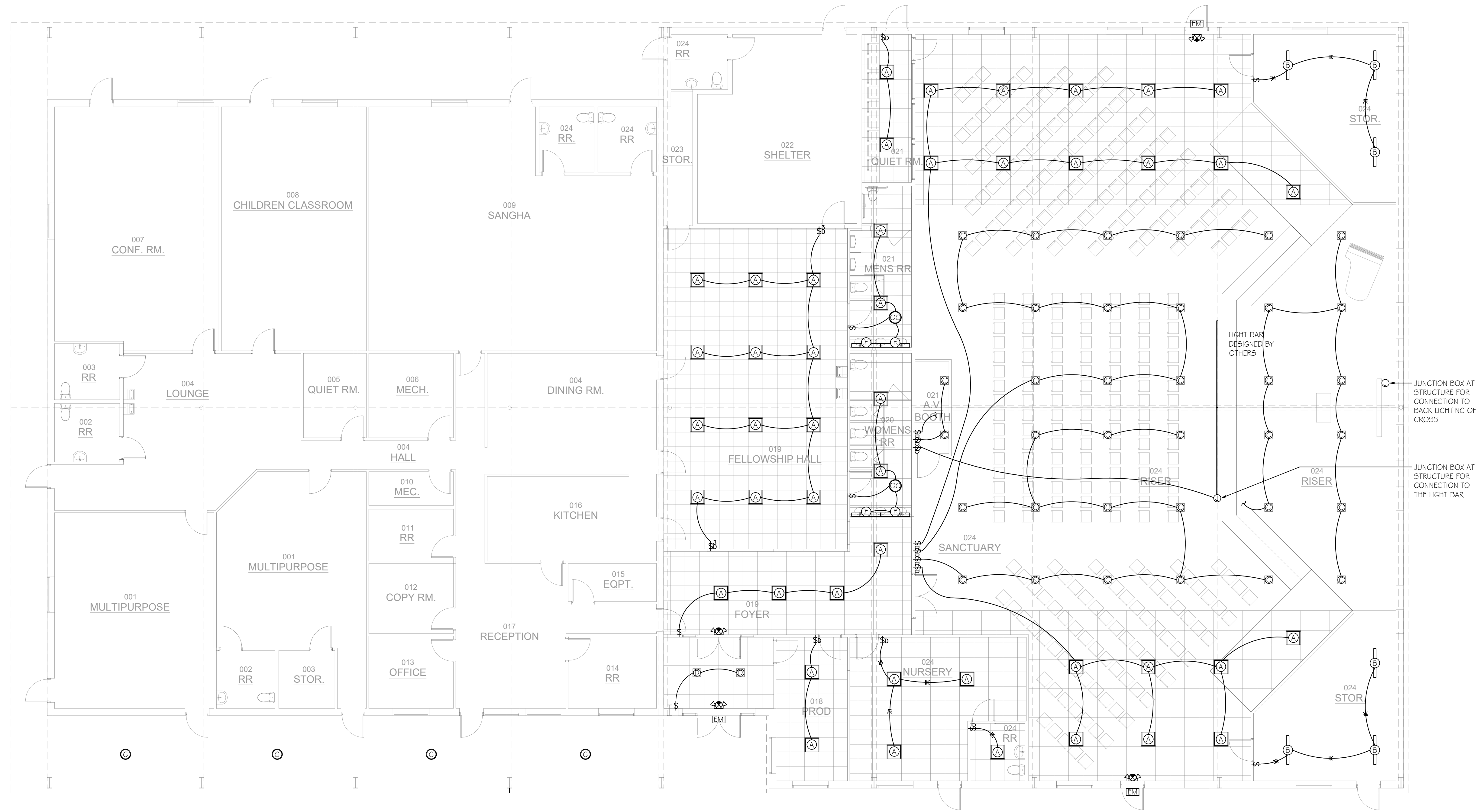
A ELECTRICAL FLOOR PLAN - LIGHTING SCALE: 1/8" = 1'-0" 0 2 4 8 16 NORTH
