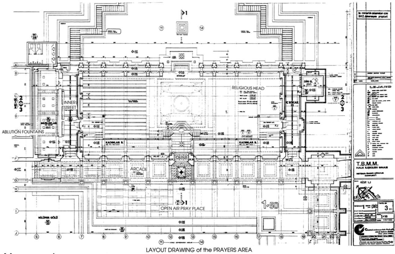
Mosque, plan
