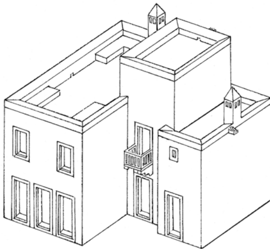
Two storey villa, plans, axonometric. IID
