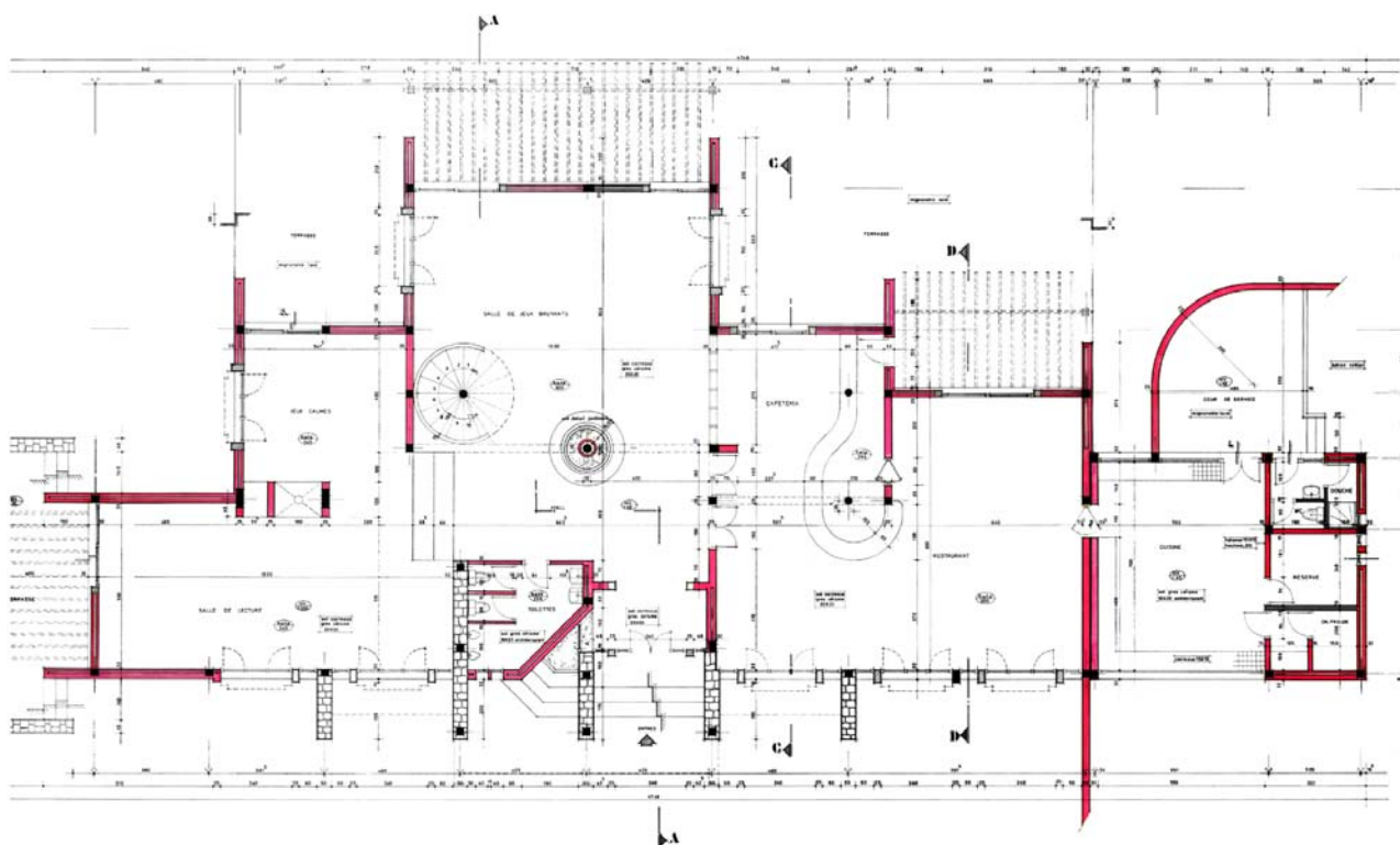
Executive club, ground floor plan
