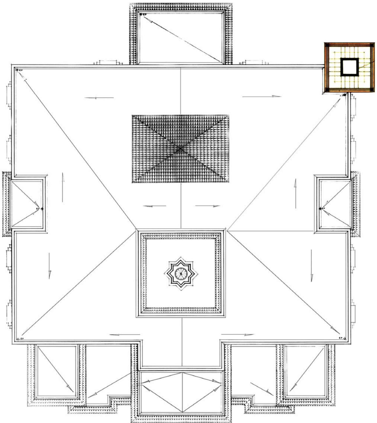
Mosque, roof plan
