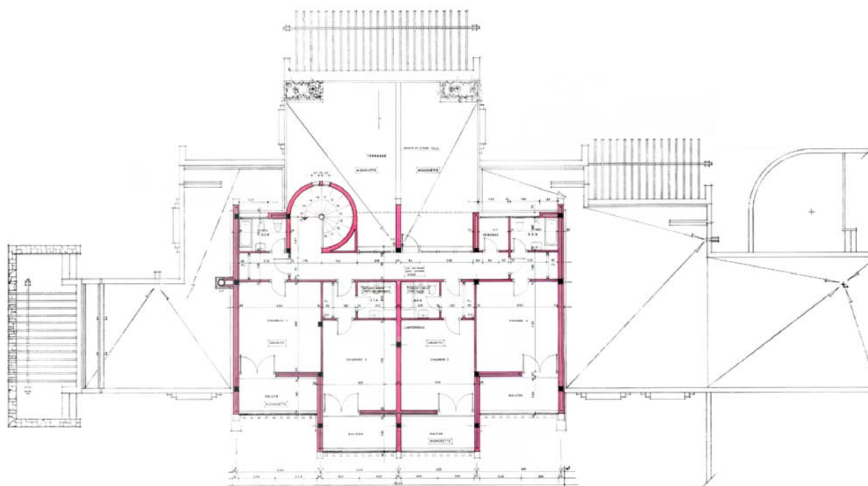
Executive club, first floor plan
