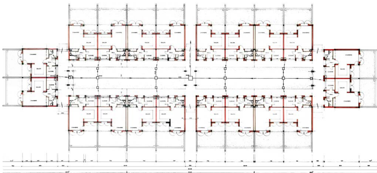
Single person housing, ground floor plan
