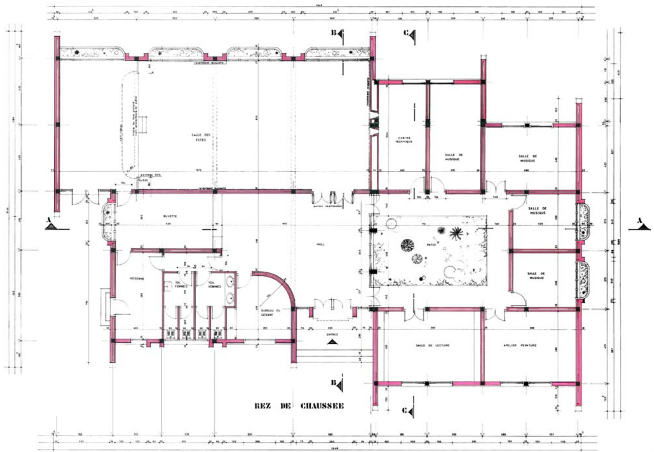
Cultural centre, ground floor plan
