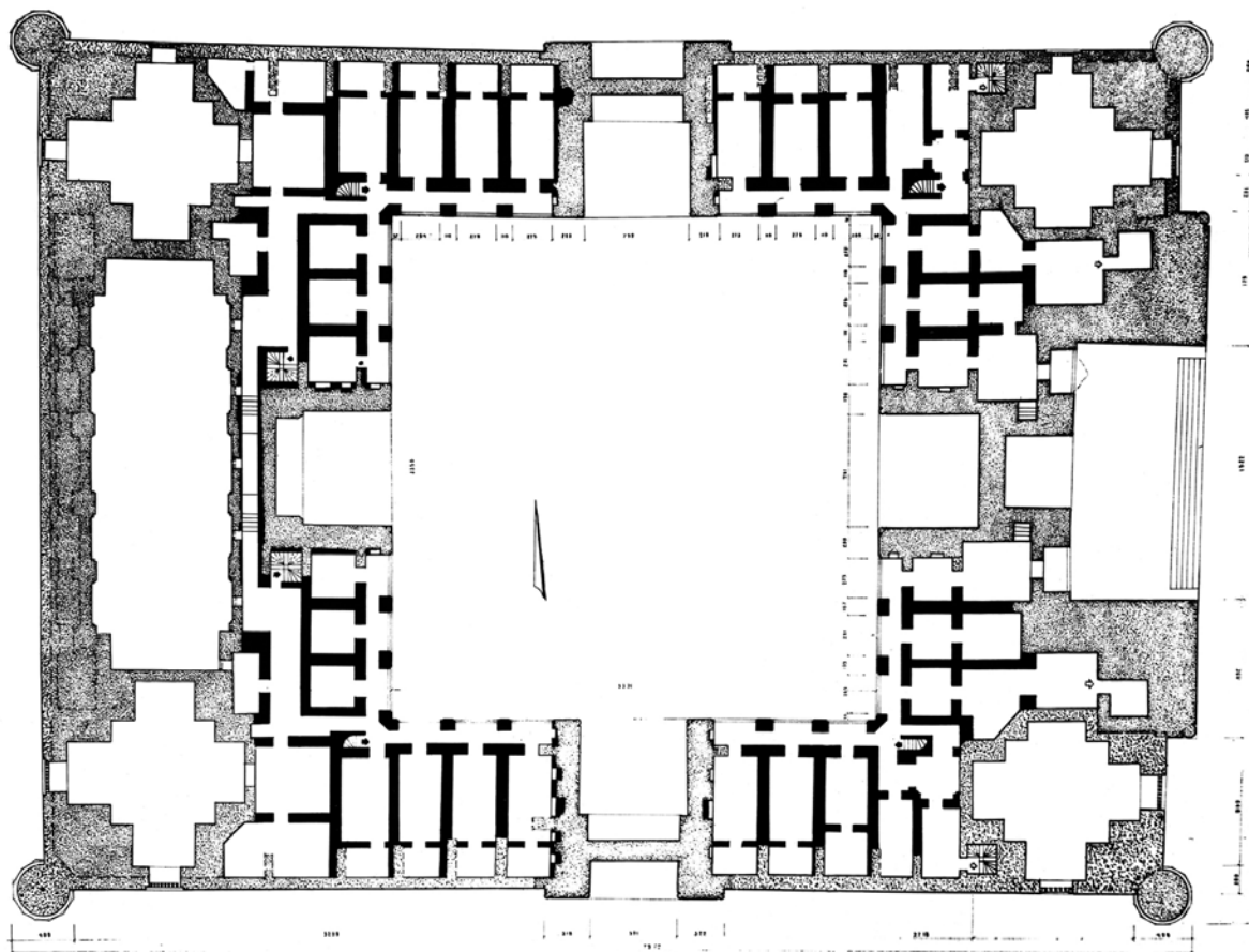
Ulugh Beg madrasa, first floor restoration proposals, 1984
