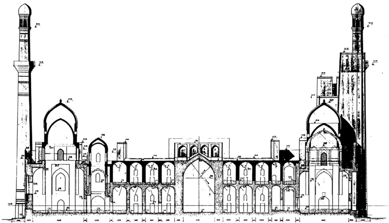
Ulugh Beg madrasa, East-West section, 1984
