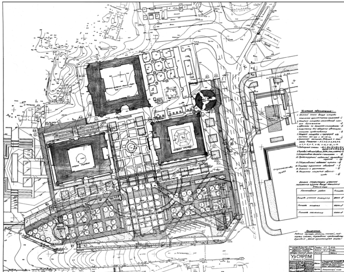
Site plan of ensemble
