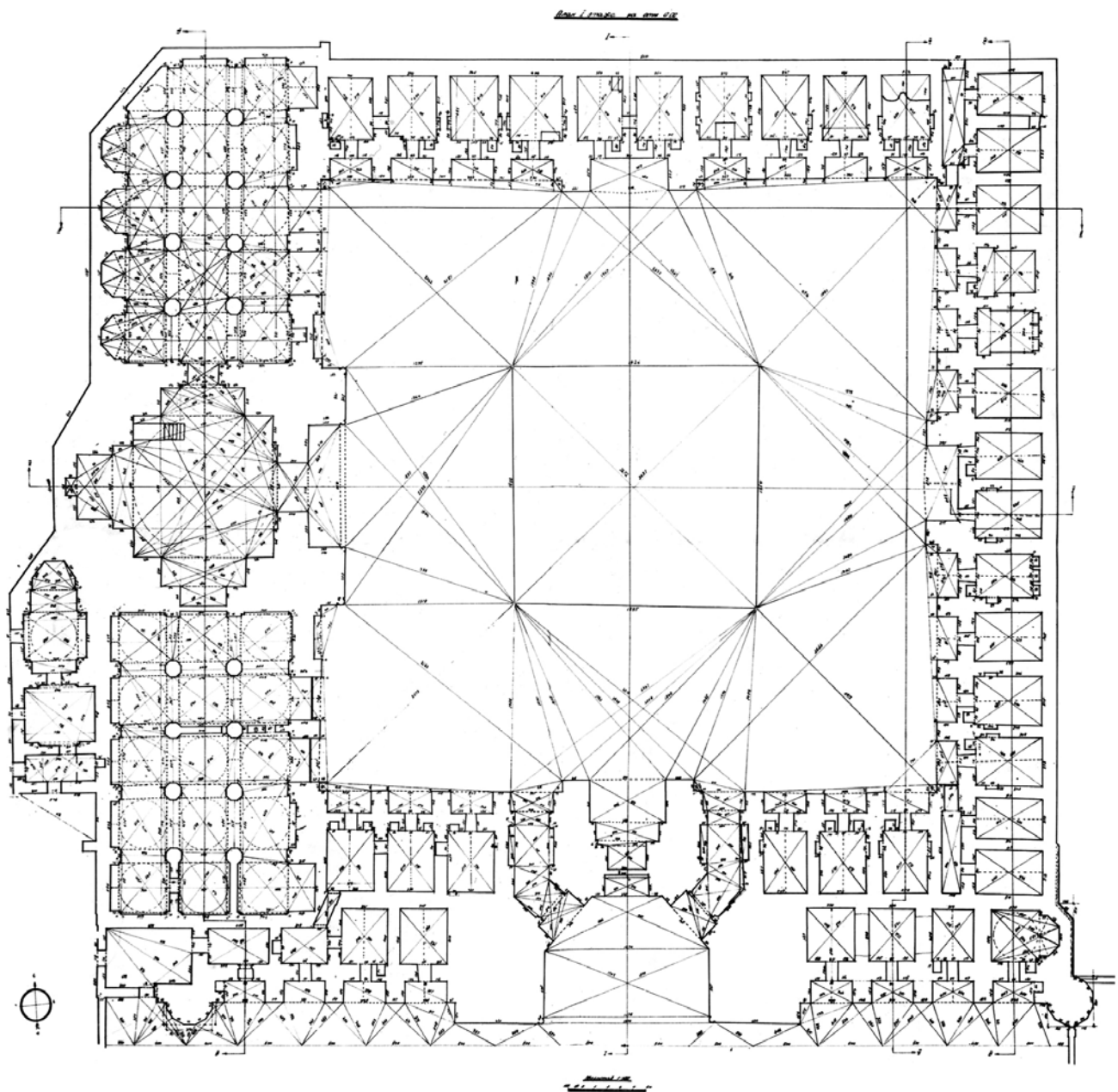
Tillya Kari madrasa and mosque, ground floor plan
