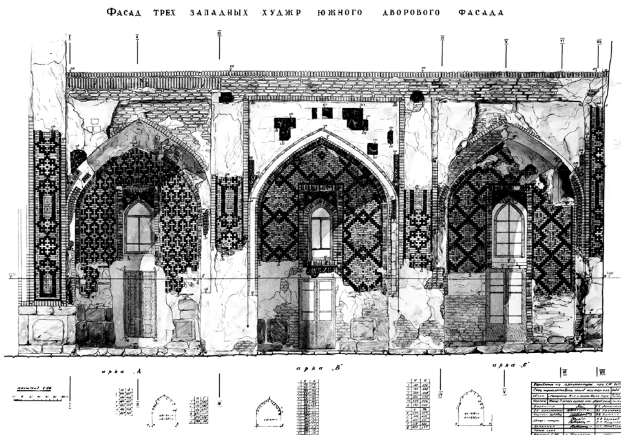
Tillya Kari madrasa and mosque courtyard, measurement draft by V. Mashchenko
