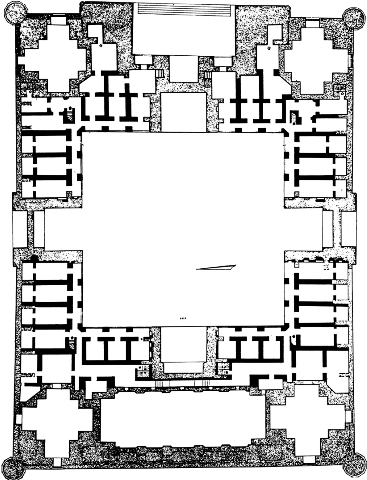
Ulugh Beg madrasa, first floor restoration proposals, 1984
