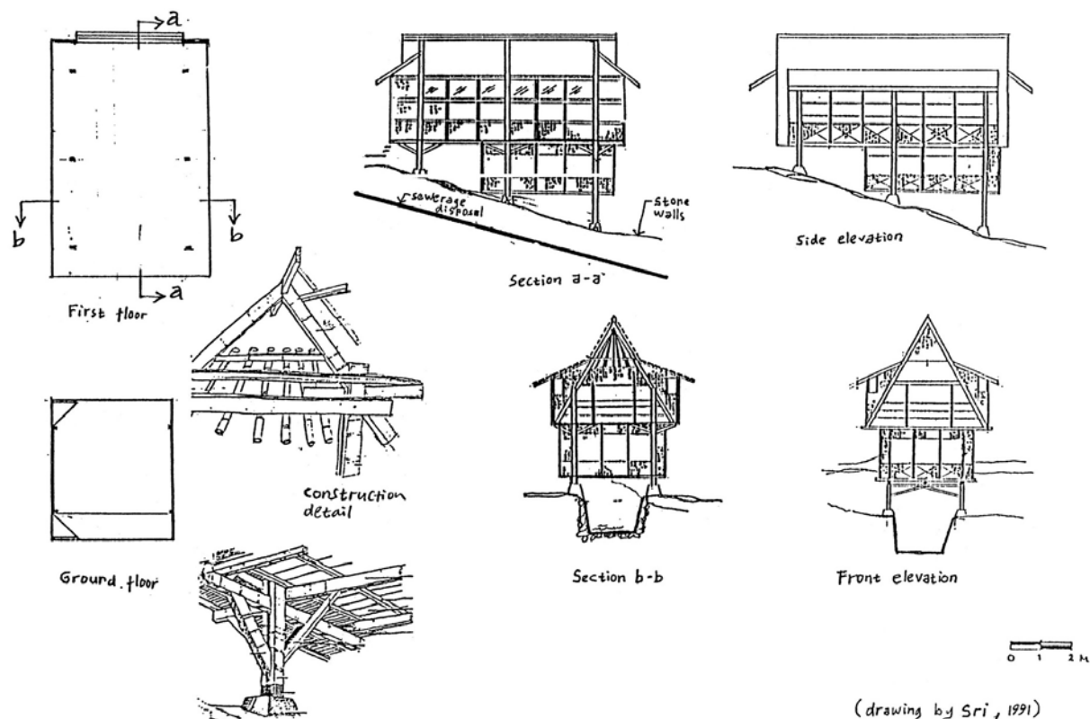
Fig. 7: House of the Brotherhood of Neighbours -
