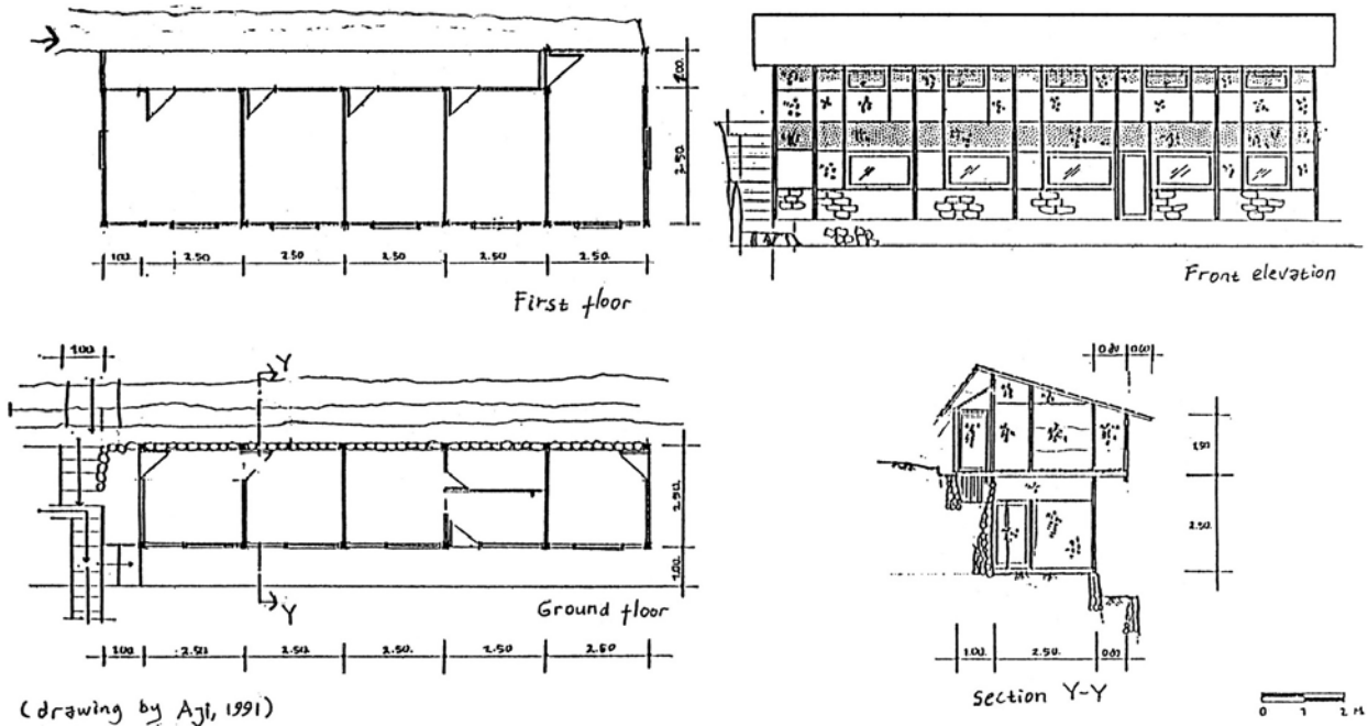
Fig. 6: Main Building Flat B
