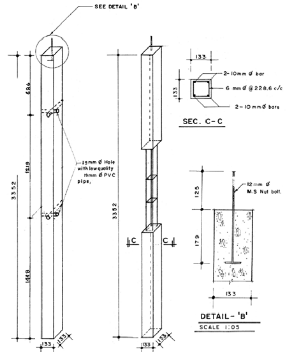
133x133 R.C.C. POST SCALE 1:20
