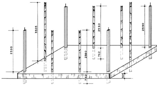
POSITION OF POST SCALE 1:50
