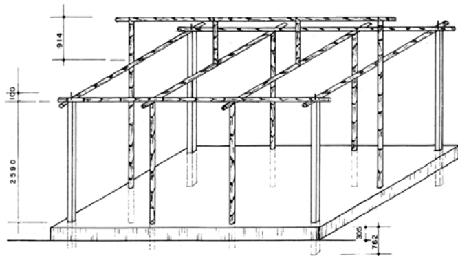
FRAME OF TIN SHED HOUSE SCALE 1:50
