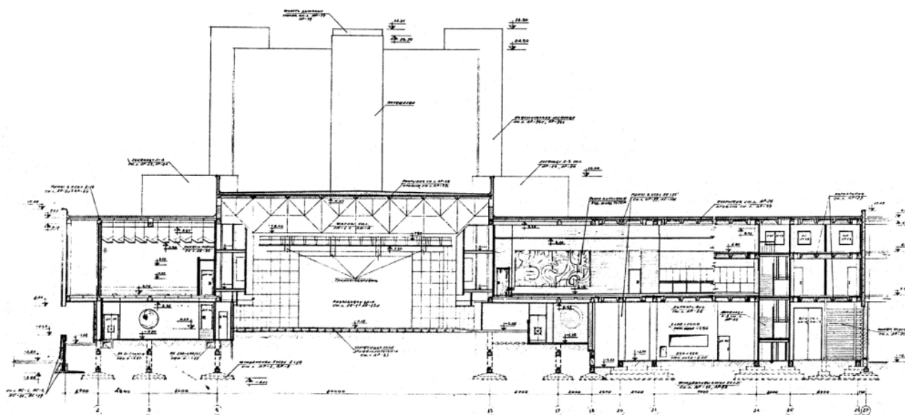
Section II - II 1:200
