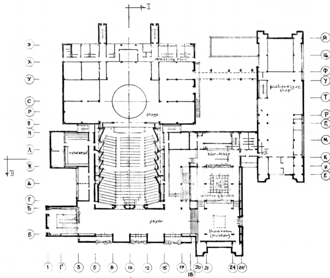
Second Floor Plan 1:400
