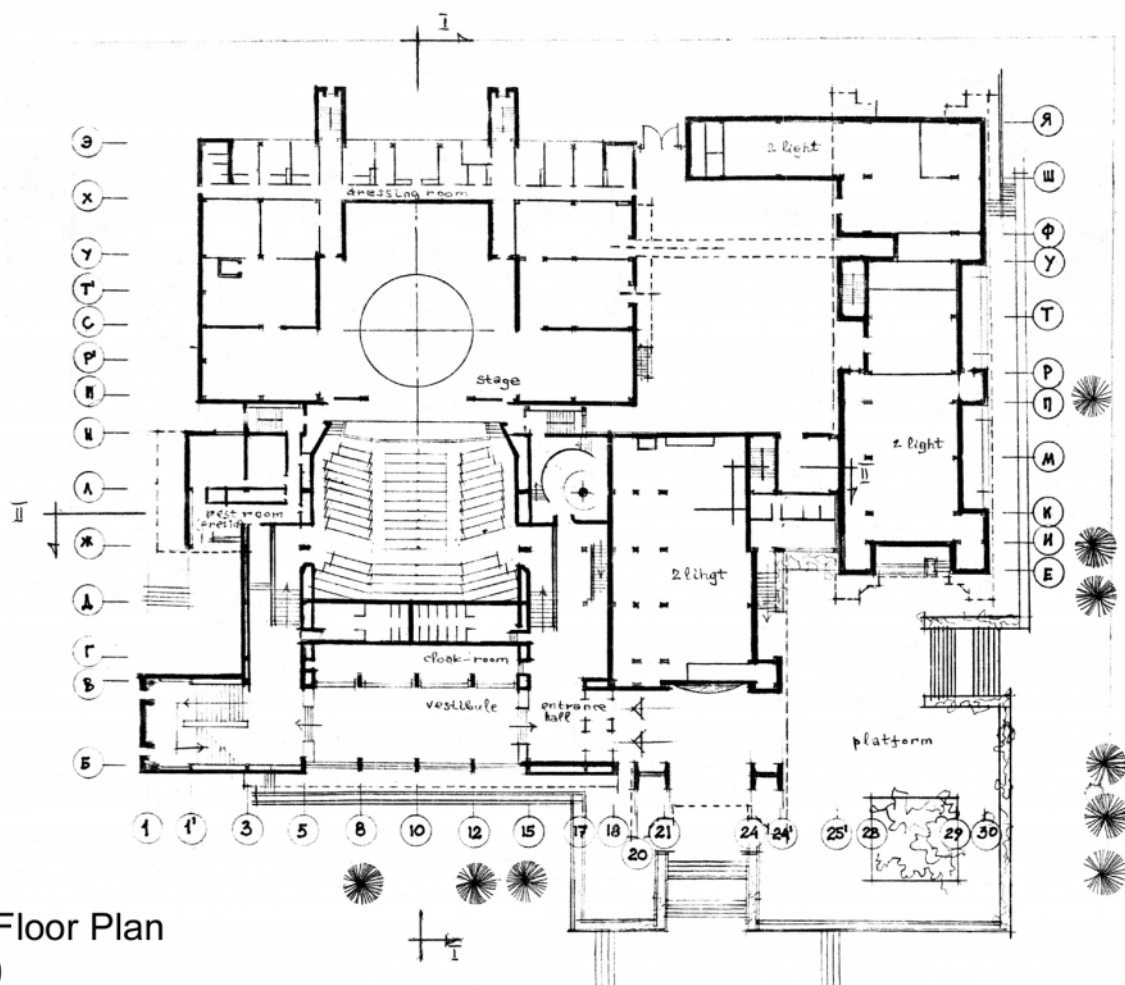
Ground Floor Plan 1:400
