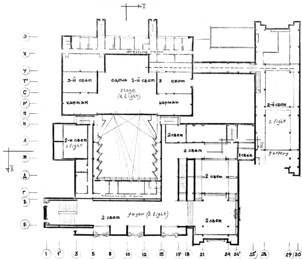
Third Floor Plan 1:400
