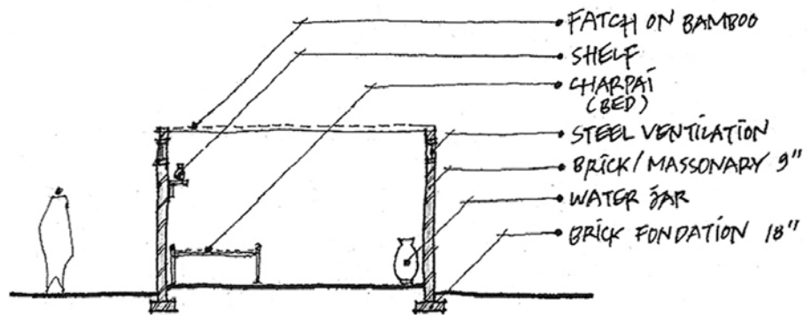
ROOM - SECTION
