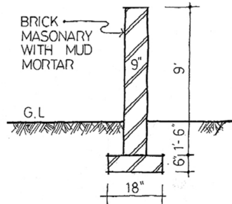
WALL SECTION
