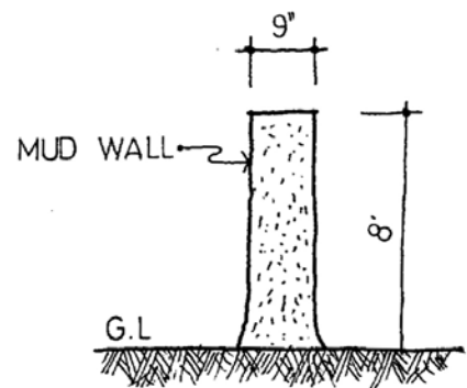
WALL SECTION
