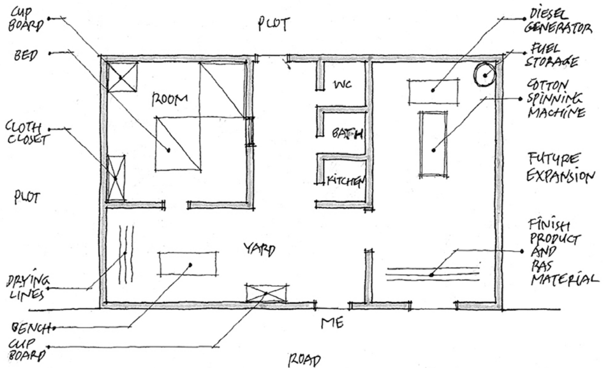
PLAN
