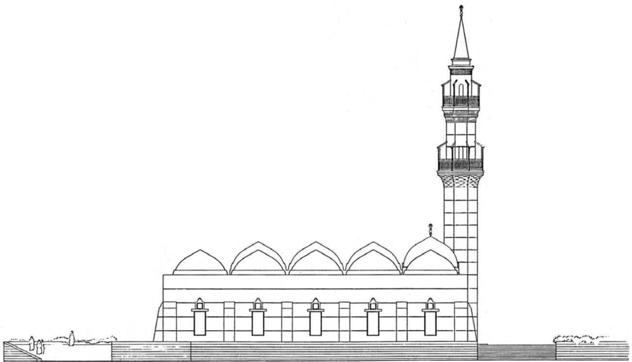
Juffali Mosque: South Elevation
