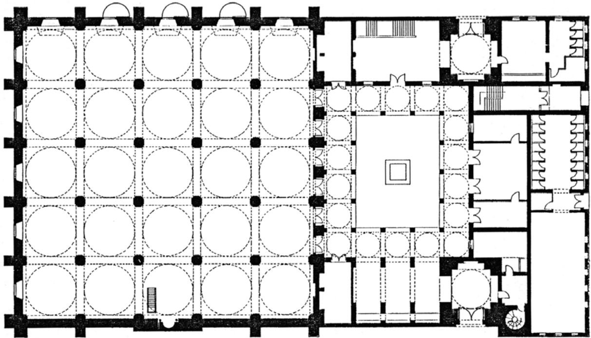
Juffali Mosque: First Floor Plan
