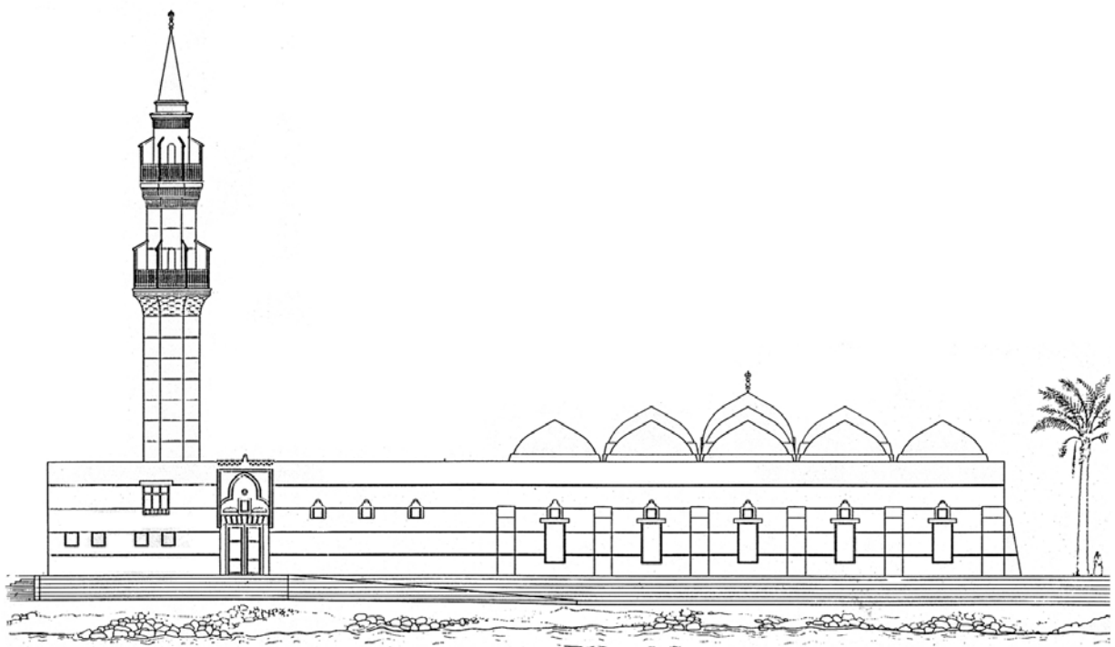
Juffali Mosque: East Elevation
