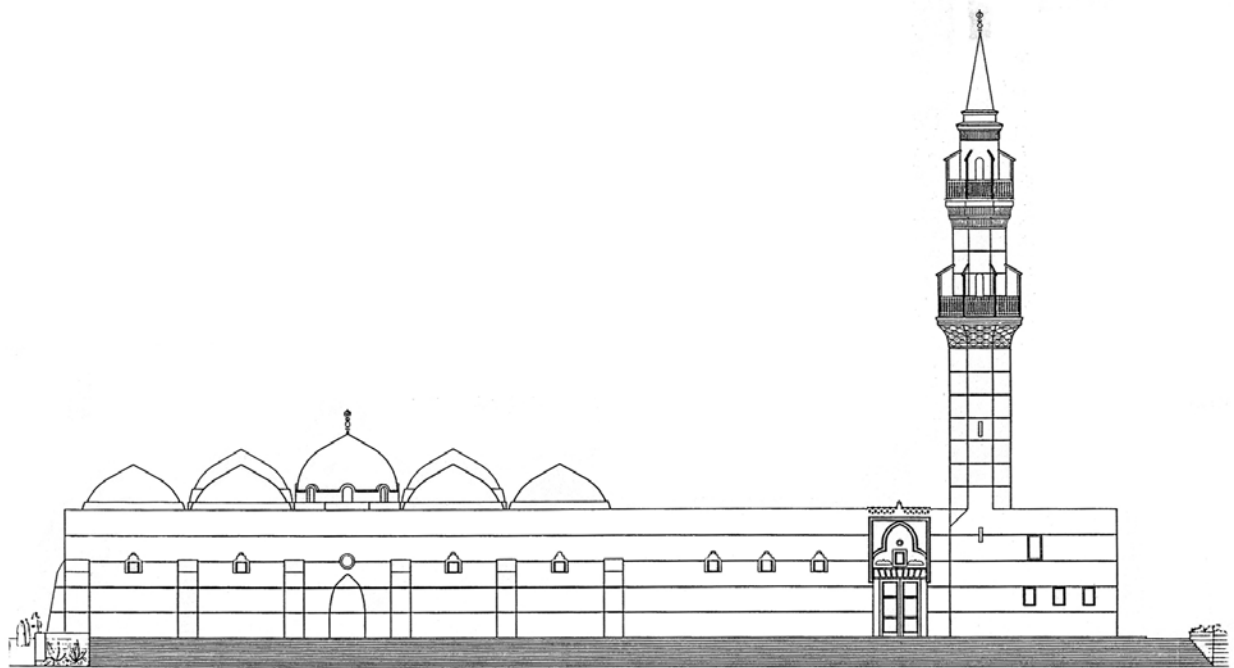
Juffali Mosque: West Elevation
