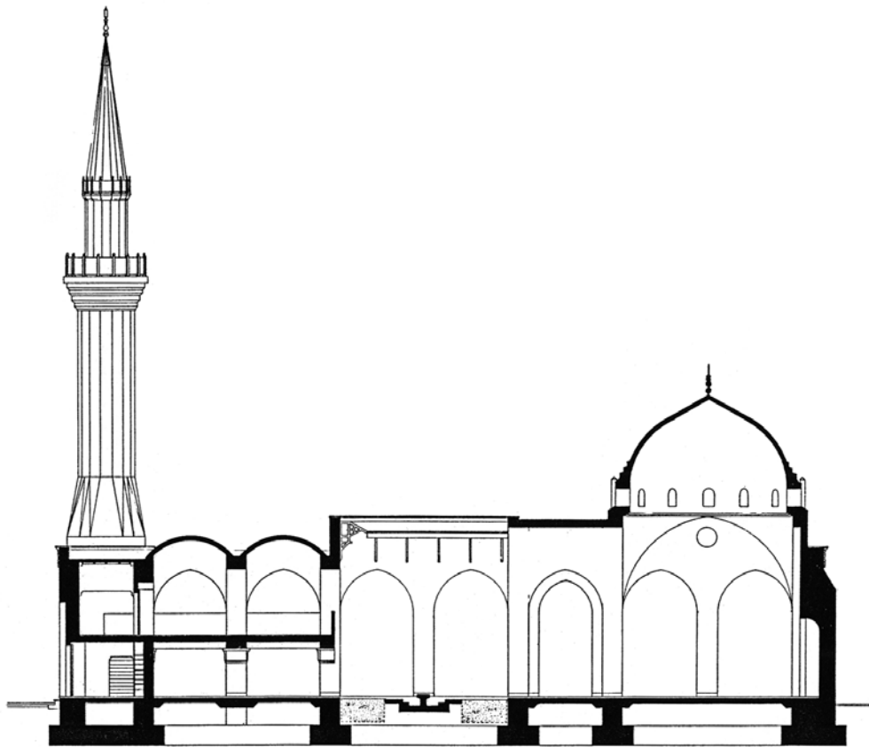
Harithy Mosque: Section
