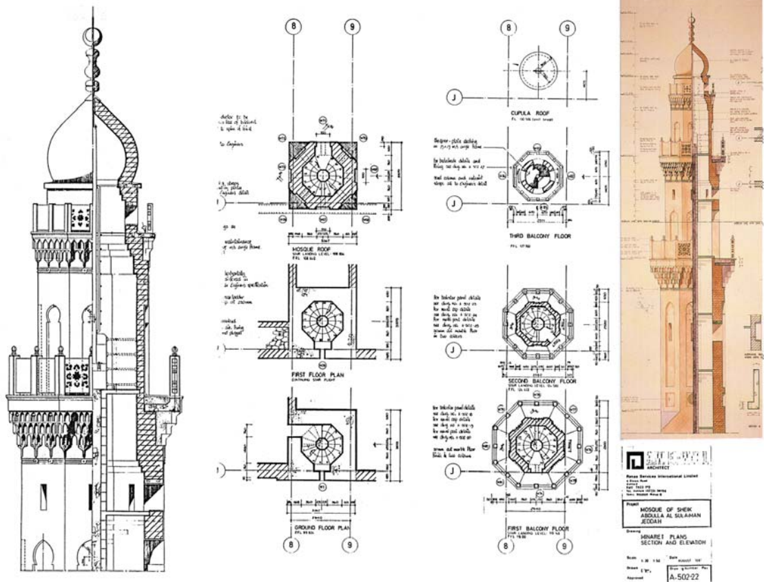
Sulaiman Mosque: Details of the Minaret
