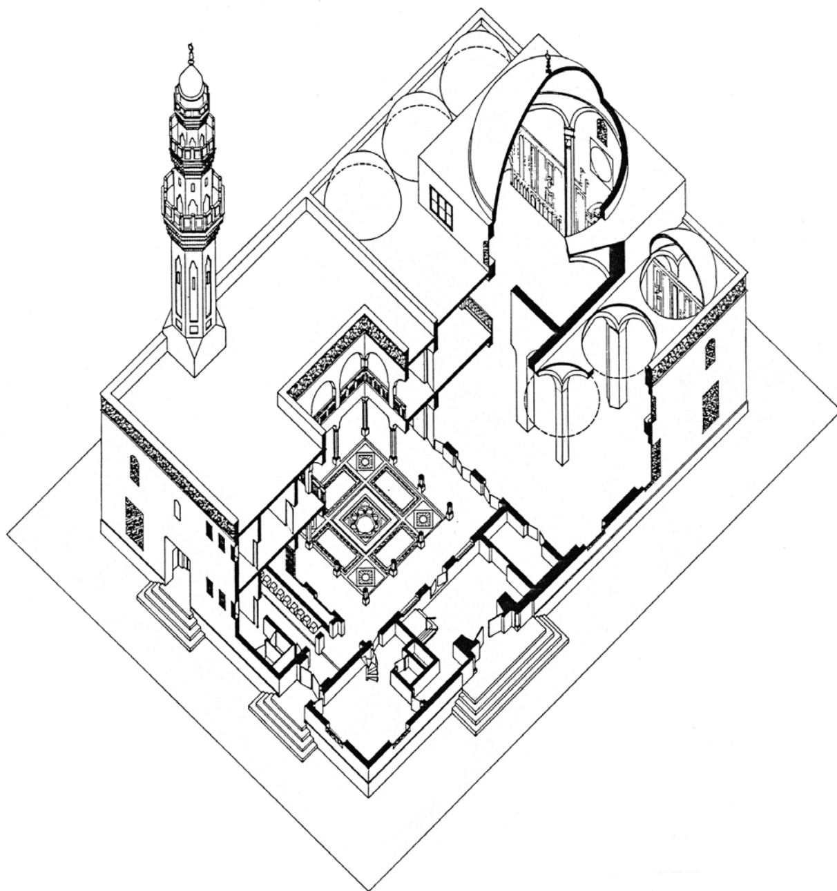
Sulaiman Mosque: Axonometric View
