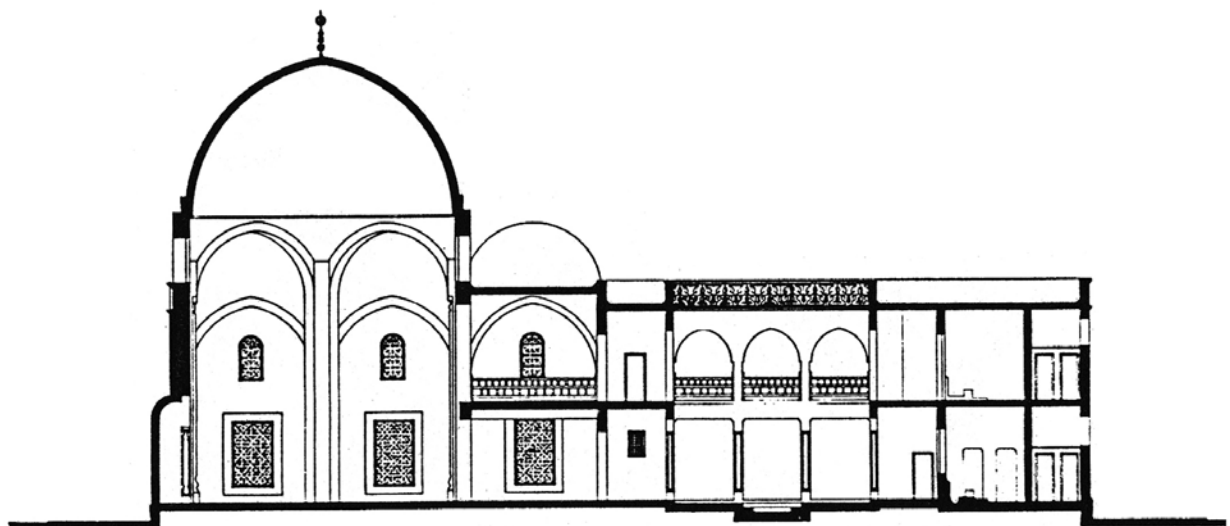
Sulaiman Mosque: Section
