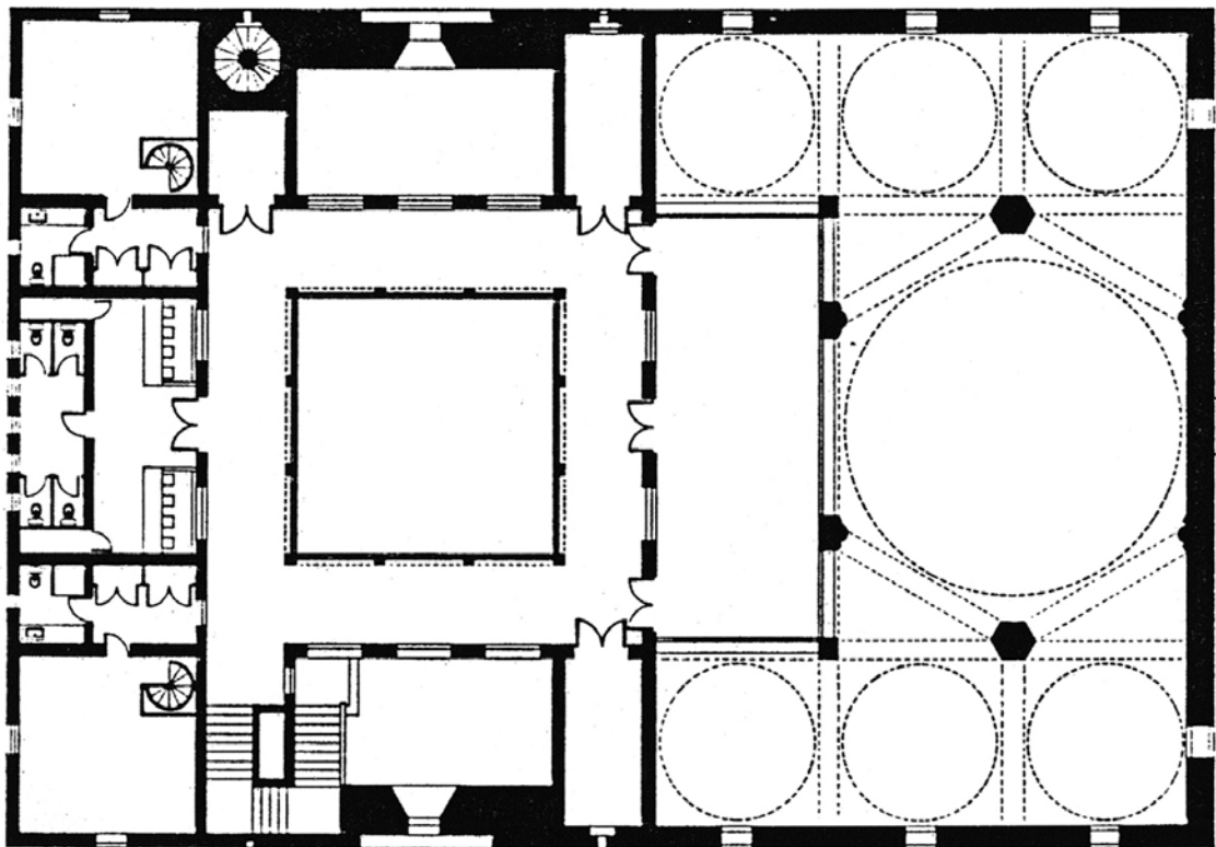
Sulaiman Mosque: Ground Floor Plan
