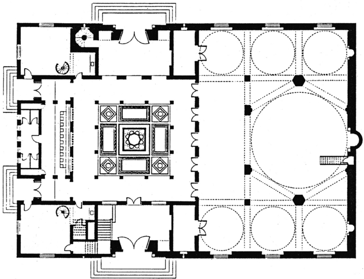
Sulaiman Mosque: First Floor Plan
