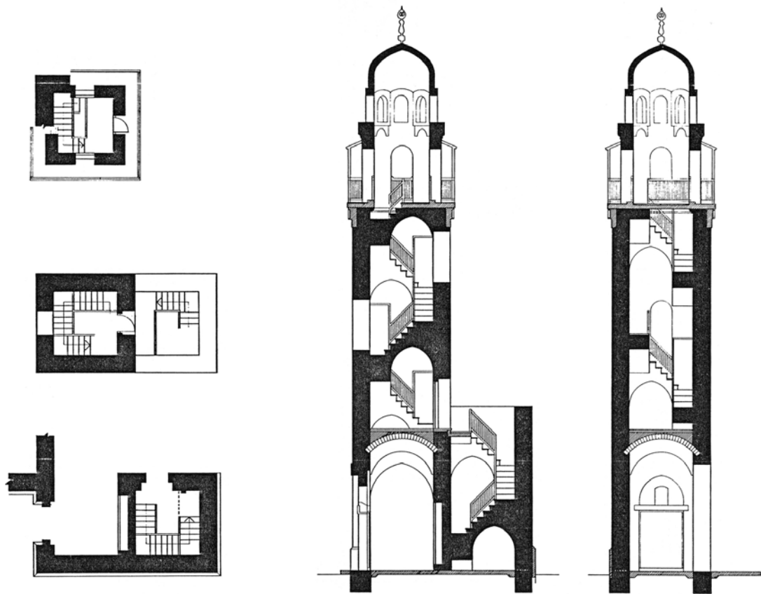
Isalnd Mosque: Plans and Sections of the Minaret
