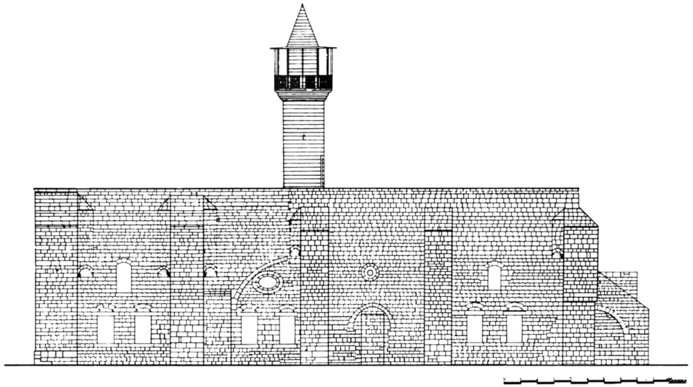
Southern Façade
