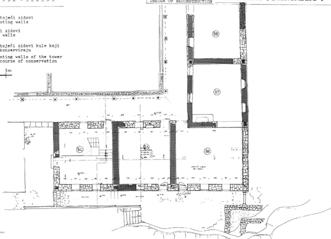
osnova prizemlja (dio) ground floor (part)
