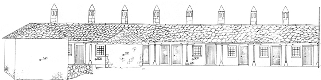
Južna fasada South facade Koski Mehmed Pašina Medresa Koski Mehmed Pasha's Madrash
