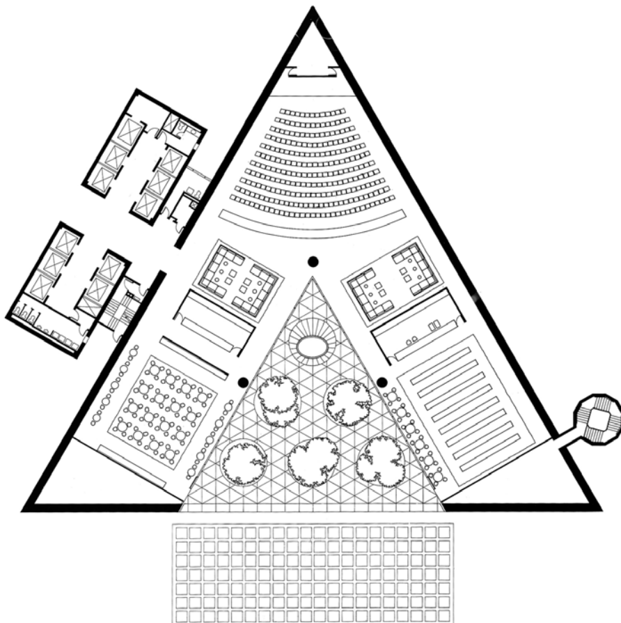
Plan: common facilities level
