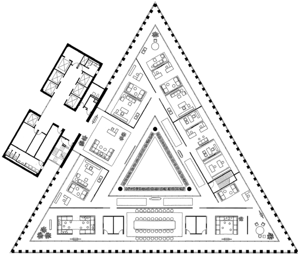
Plan: executive level
