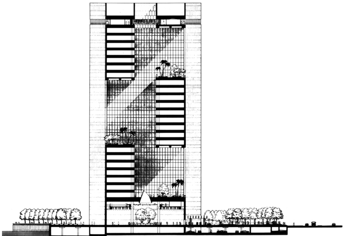
THE NATIONAL COMMERCIAL BANK JEDDAH, SAUDI ARABIA 29 JULY, 1978 SECTION SKIDMORE, OWINGS & MERRILL ARCHITECTS
