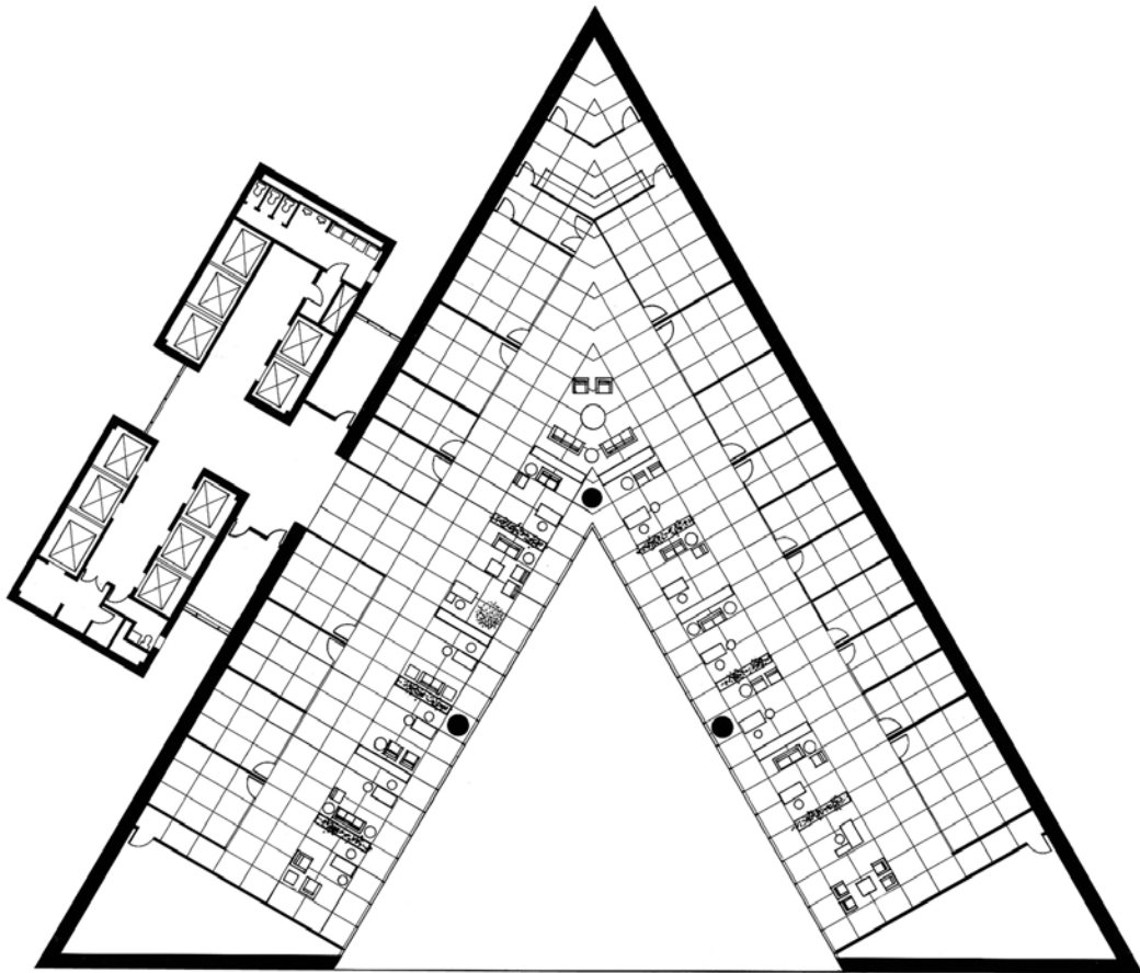
Plan: typical office level
