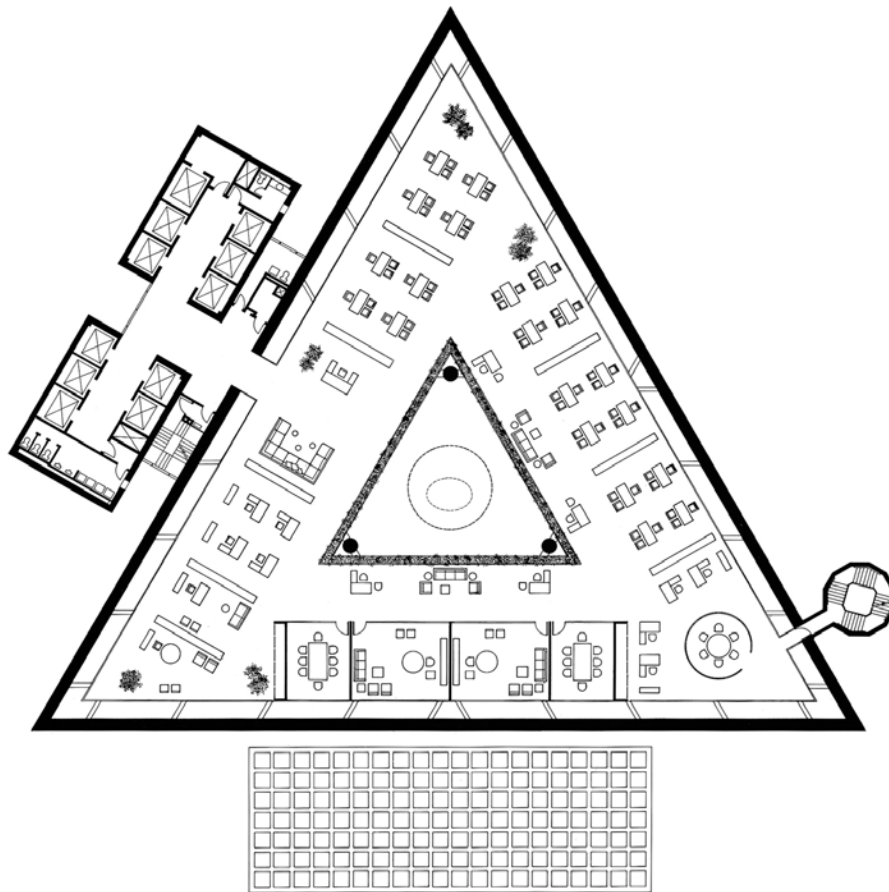
Plan: mezzanine level
