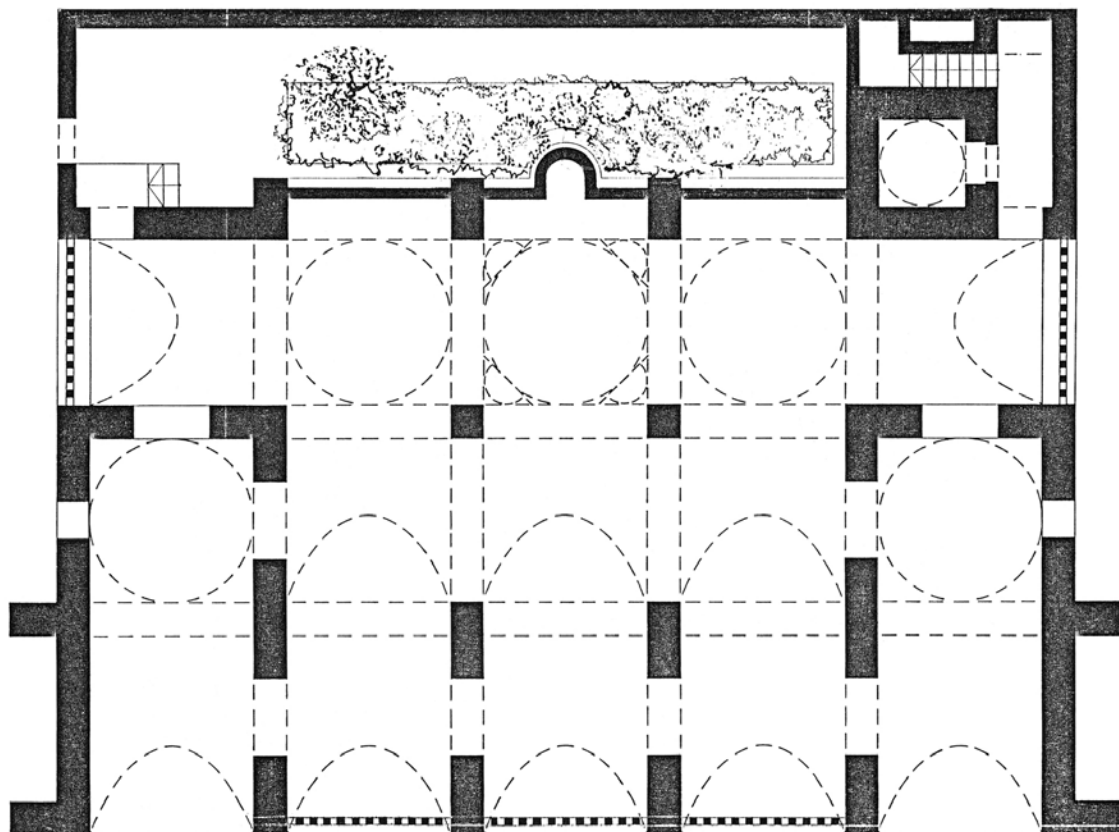
Ruwais Mosque: Plan
