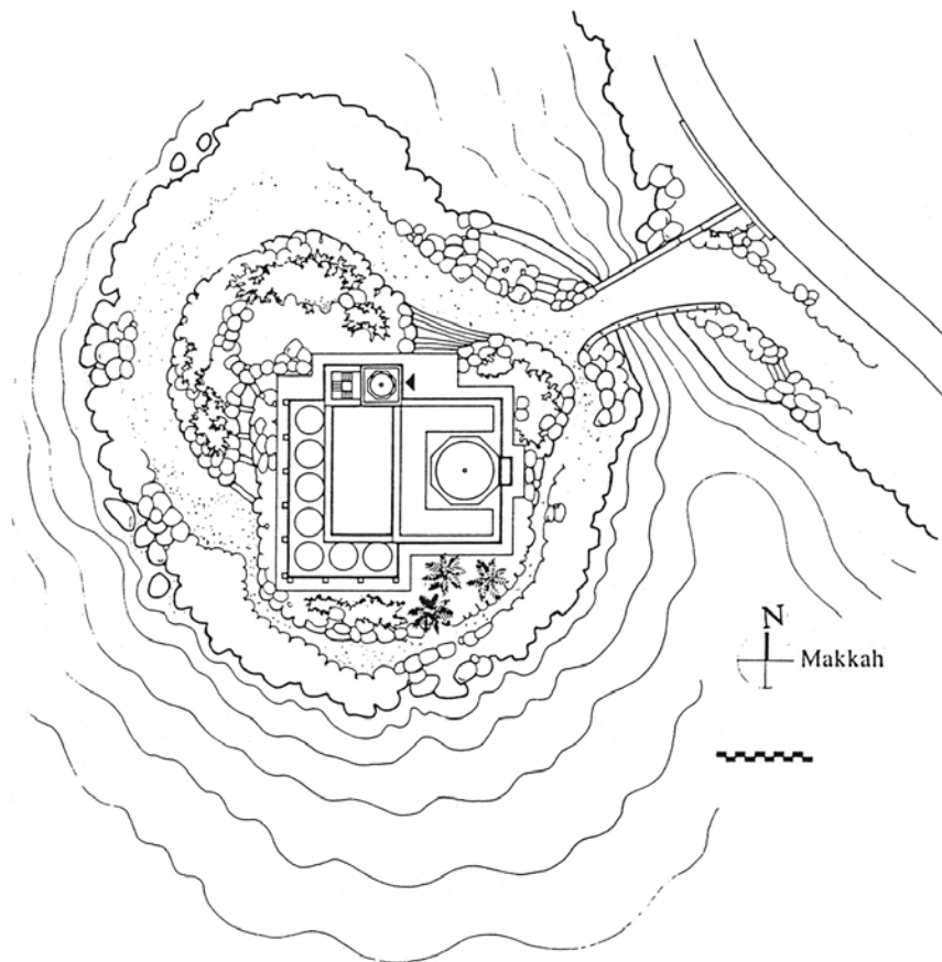
Island Mosque: Site Plan
