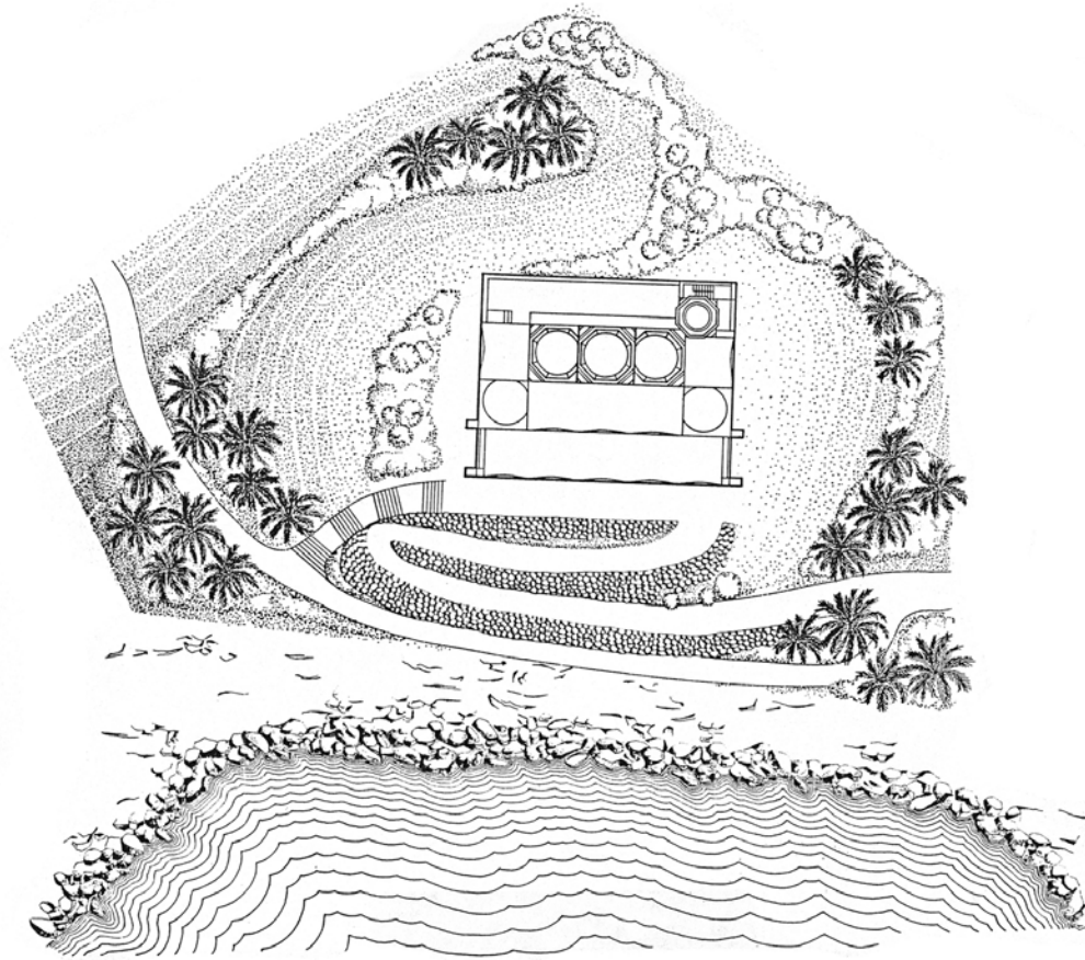
Ruwais Mosque: Site Plan
