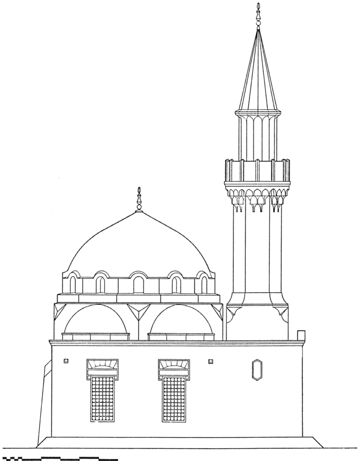
Binladen Mosque: North Elevation
