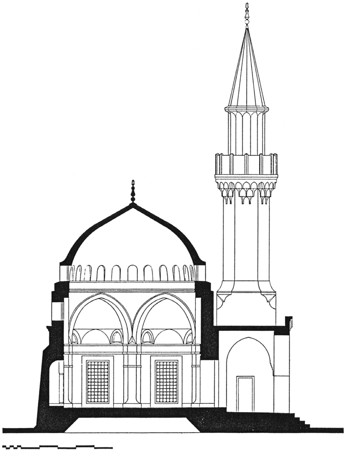
Binladen Mosque: Section
