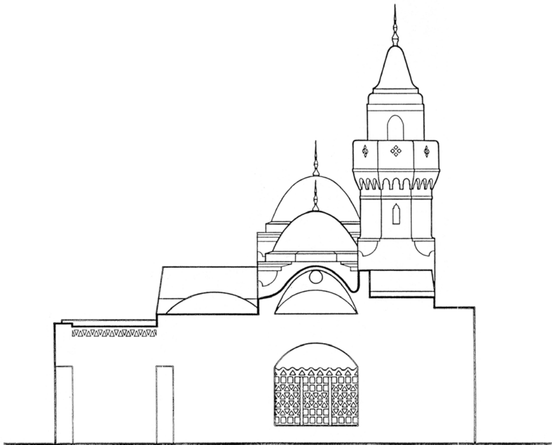
Ruwais Mosque: South Elevation
