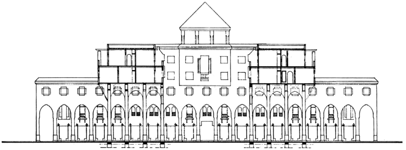
Section through gallery connecting two blocks of apartments; elevations of apartment blocks.
