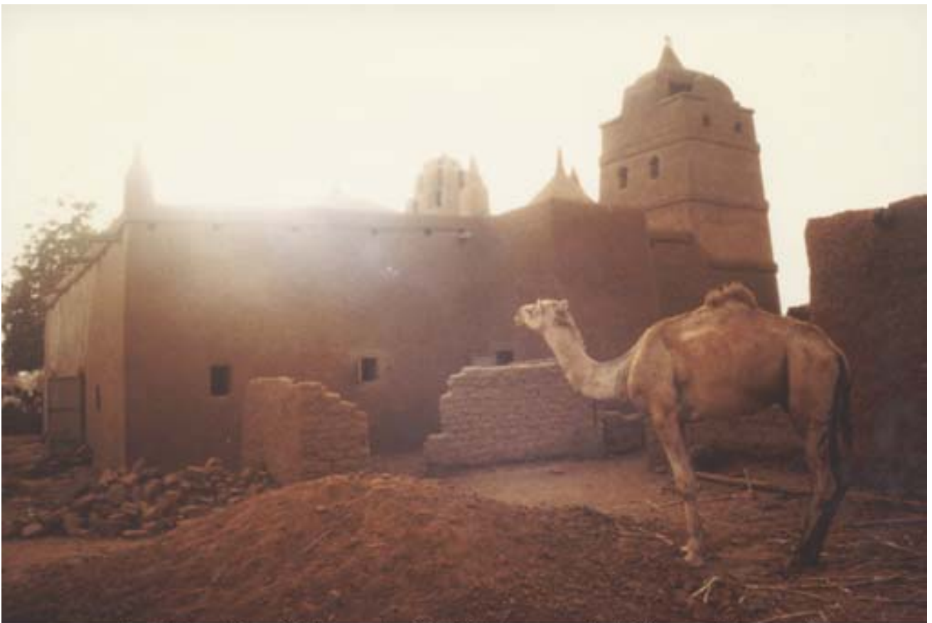
East elevation, Qibla wall of Tajaé Mosque (not Yamaa Mosque)
