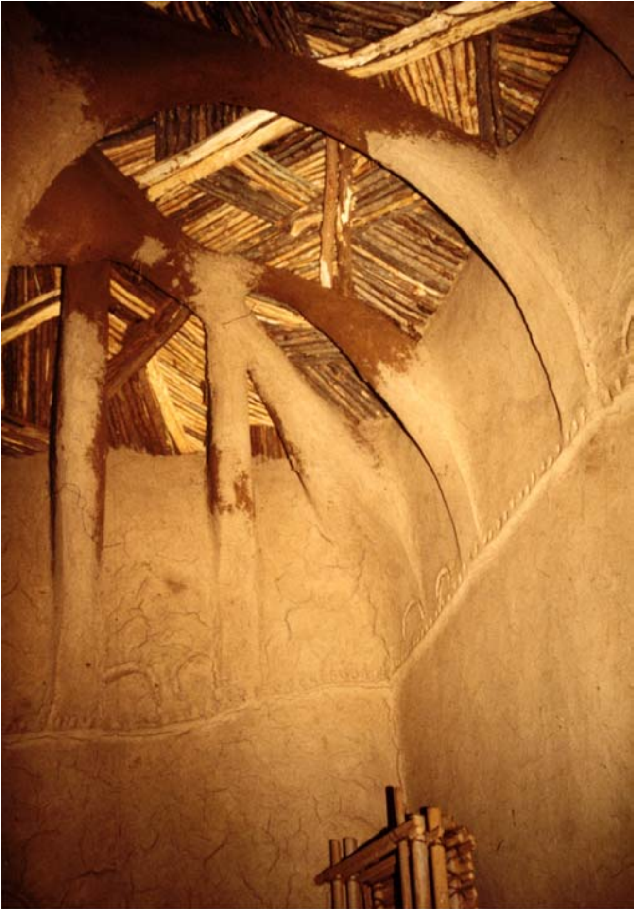
Tajaé Mosque, roofing support in corner (not Yaama Mosque, although identical to it)
