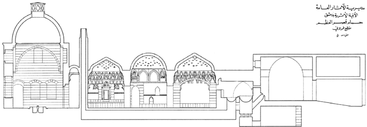
Long section through private bath
