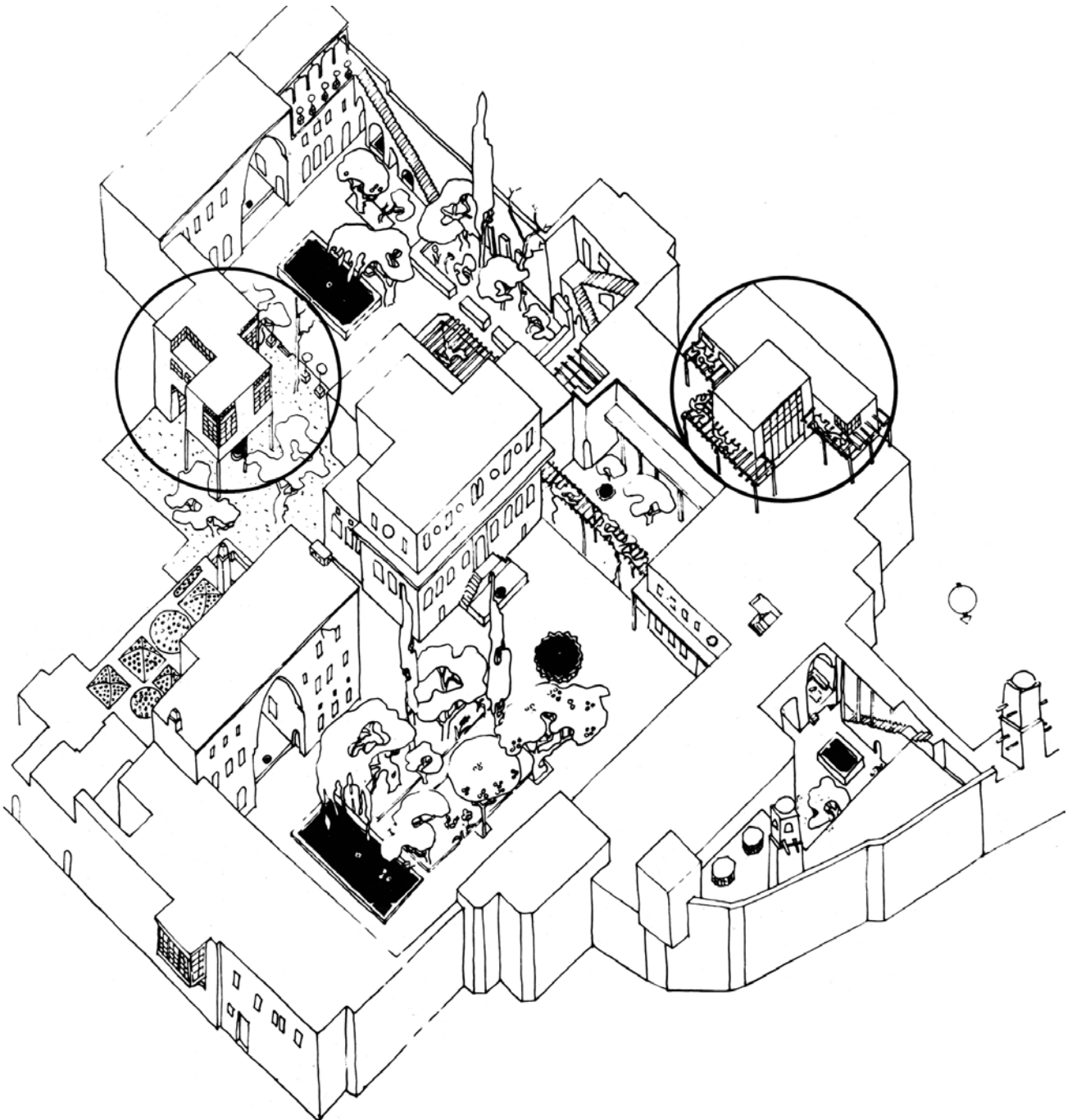
Michel Ecochard's drawing of 2 proposed dwellings for staff of French Insitue Only that on the left was built (c.1935)
