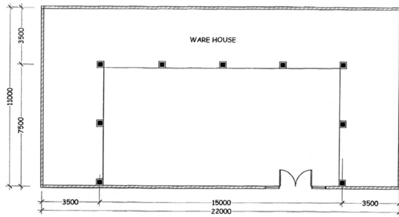
WARE HOUSE SCALE 1:100
