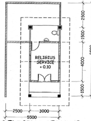
RELIGIUS SERVICE SCALE 1:100
