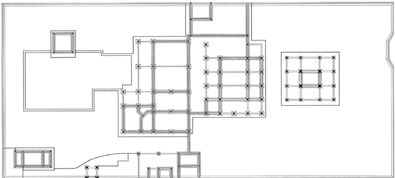
PILING PLAN SCALE 1: 200
