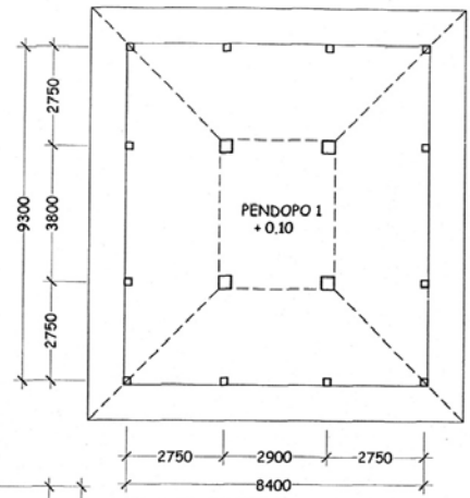
PENDOPO 1 SCALE 1:100
