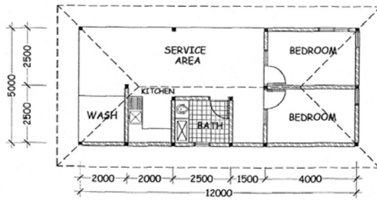
SERVICE AREA SCALE 1:100
