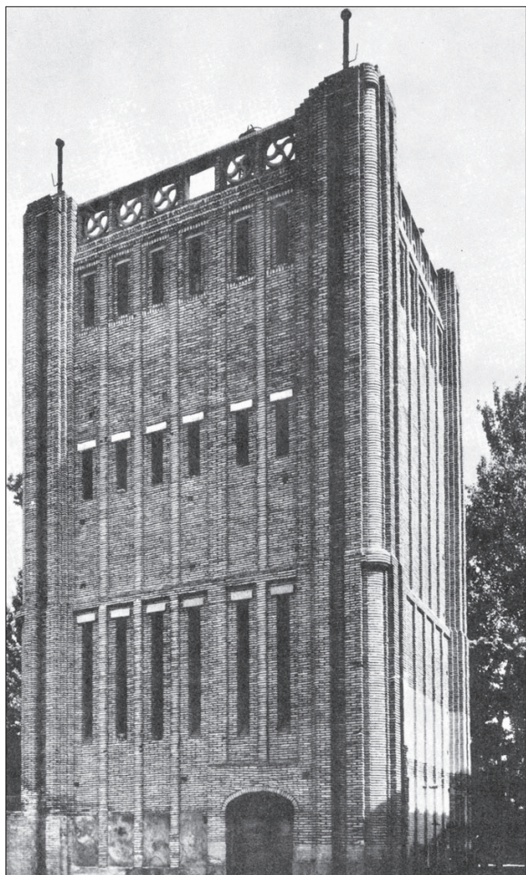
Fig. 10: Risbaf Spinning Factory, cooling tower.
