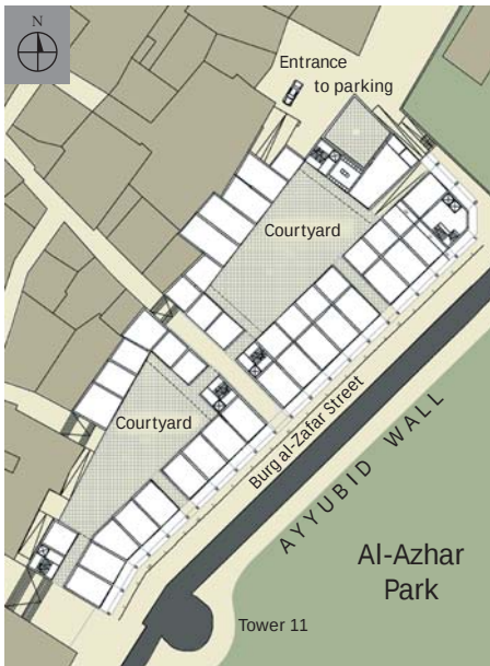
(Above) Ground floor plan of the proposed mixed-use development showing the commercial portico along Burg al-Zafar Street. Shops surround the two interior courtyards.
