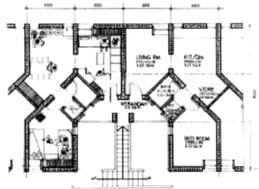
FIRST FLOOR PLAN A-TYPE UNIT (AREA - 45.00 sq.mt.)
