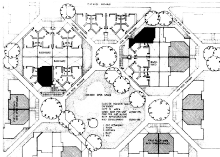
SITE PLAN
