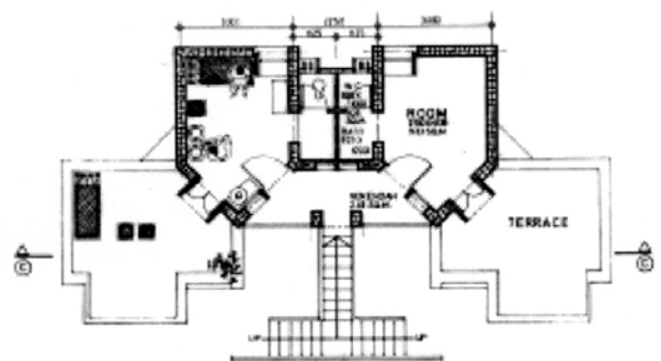
FIRST FLOOR PLAN C-TYPE UNIT (AREA - 45.00 sq.mt.)
