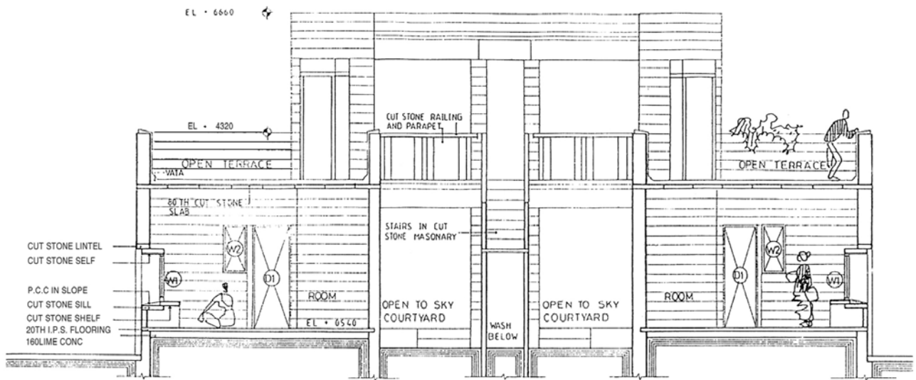
SECTION C1 TYPE UNIT Scale 1:50
