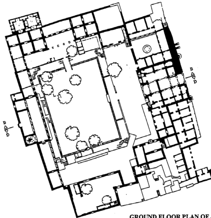
GROUND FLOOR PLAN OF JAMDAR SINGH HAVELI
