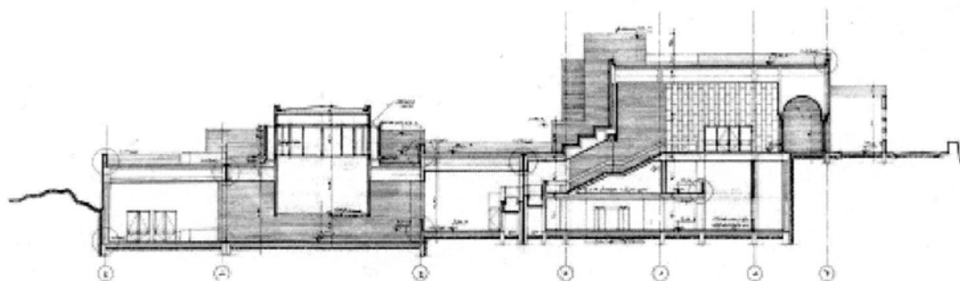
SECTION THROUGH MAIN EXHIBITION HALL
