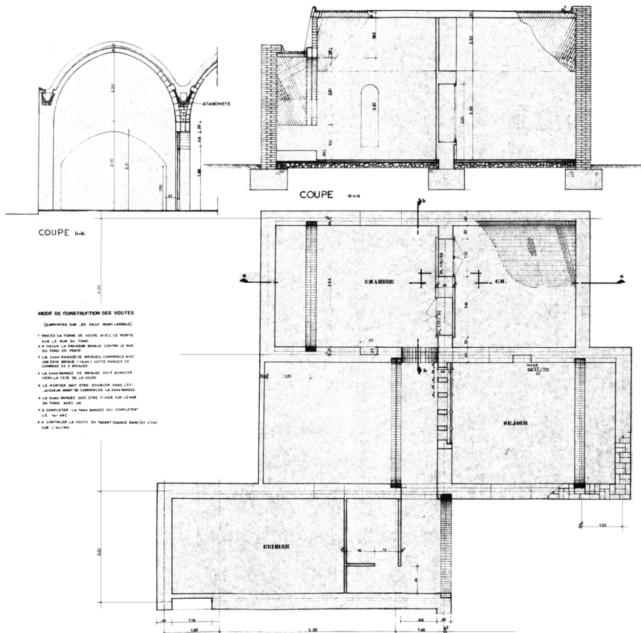
Vault construction details
