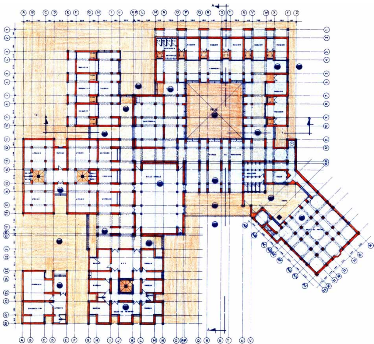
Ground floor plan: mosque, meeting rooms, post office, shops
