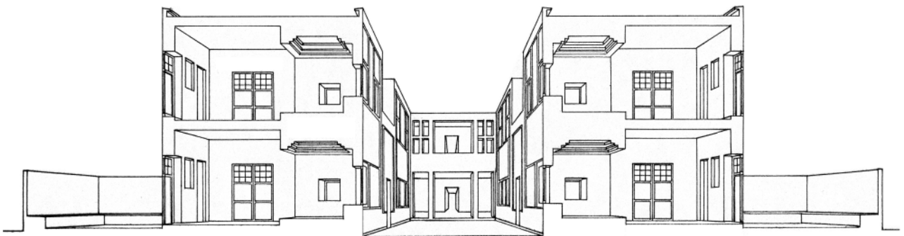
Sectional perspective through interior court and apartments units
