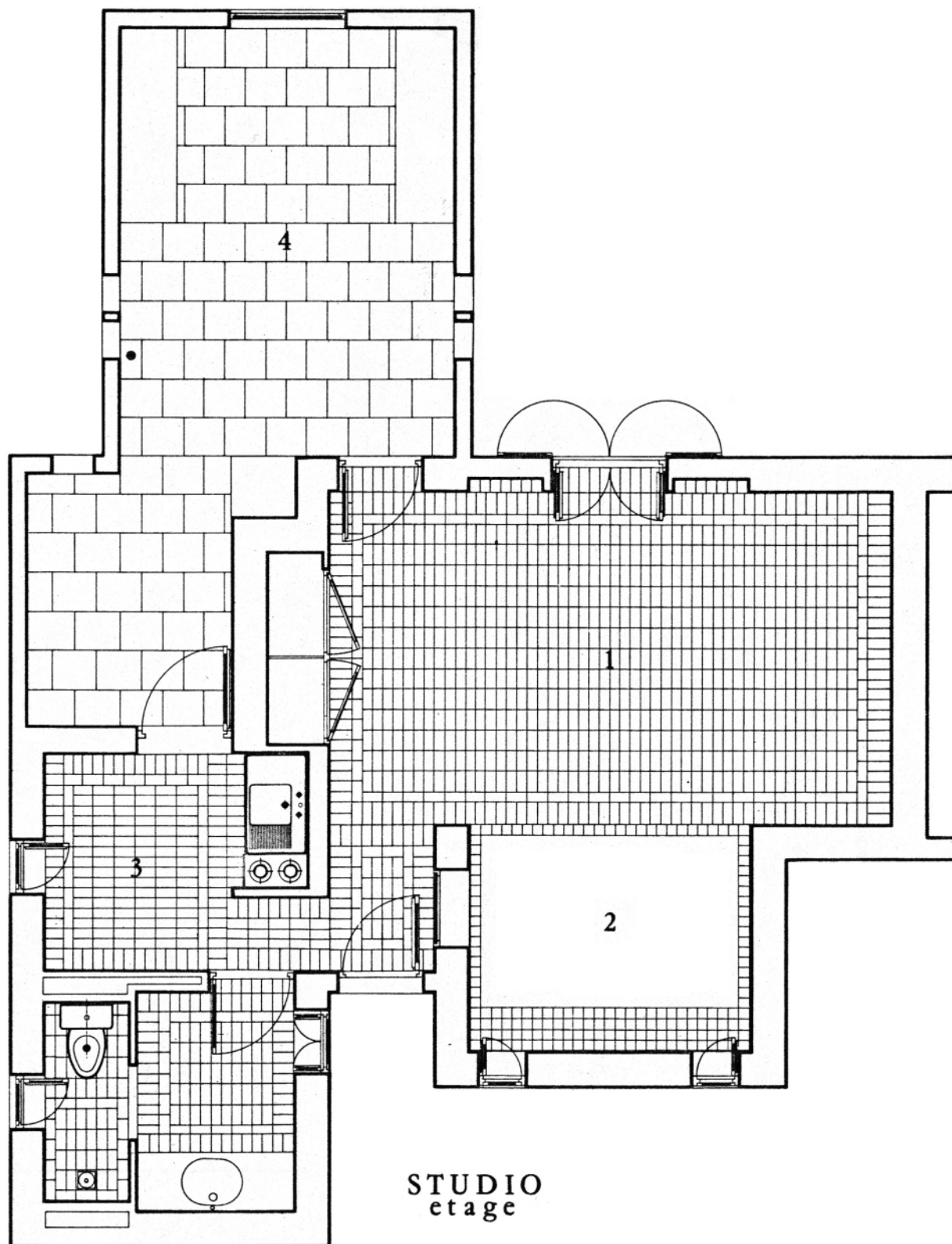
One-room apartment plan, ground floor
