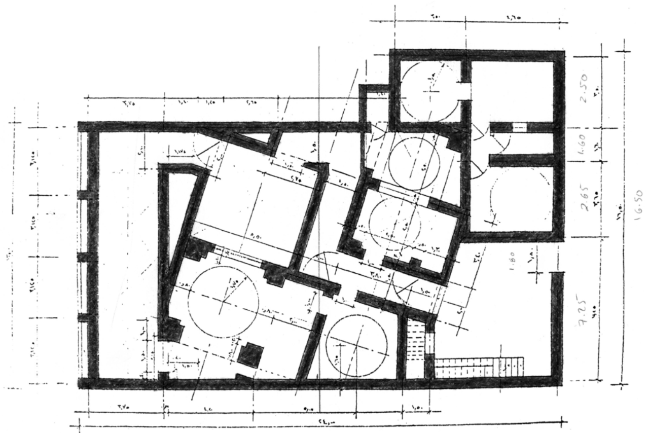
Habib Georgy Sculpture Museum: plan at ground level
