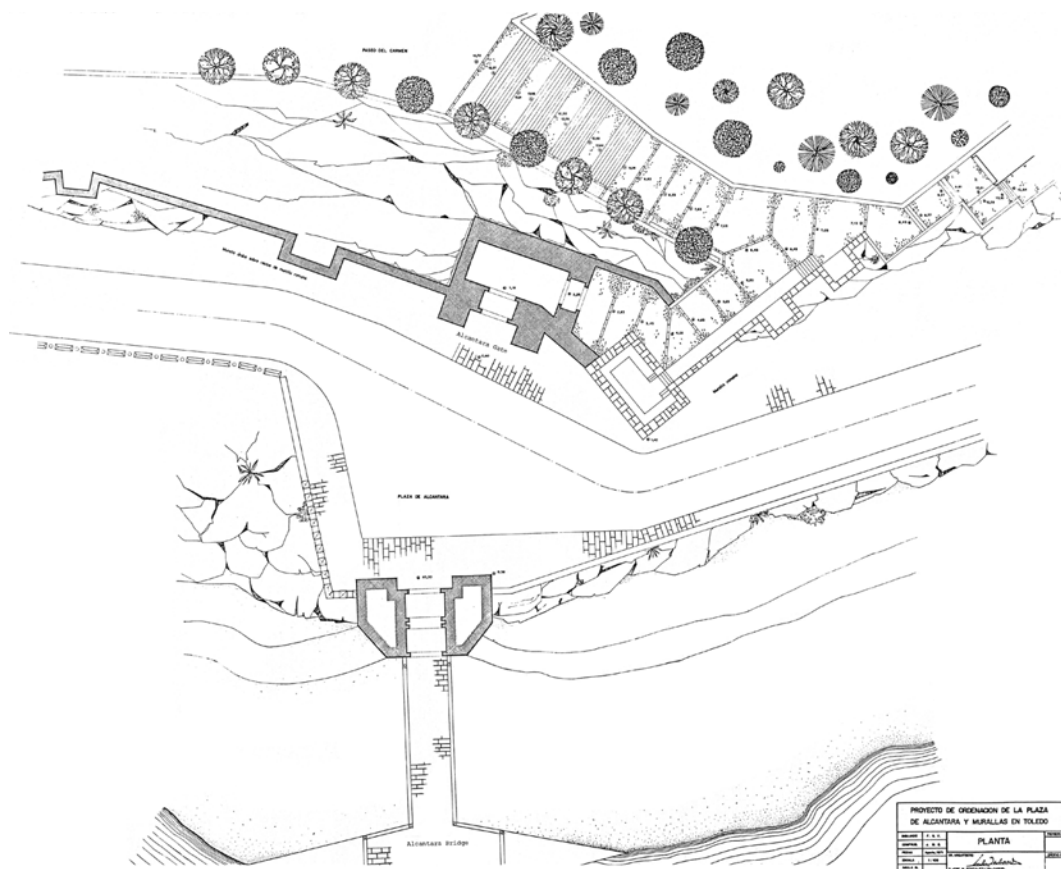
Existing Site Plan (before restoration and landscaping) Immediate environs of Monastery
