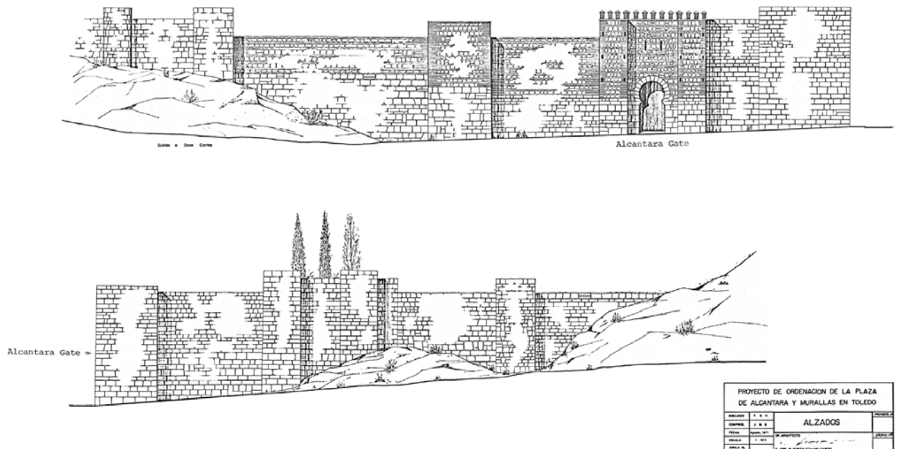
Alcantara Gate Elevations
