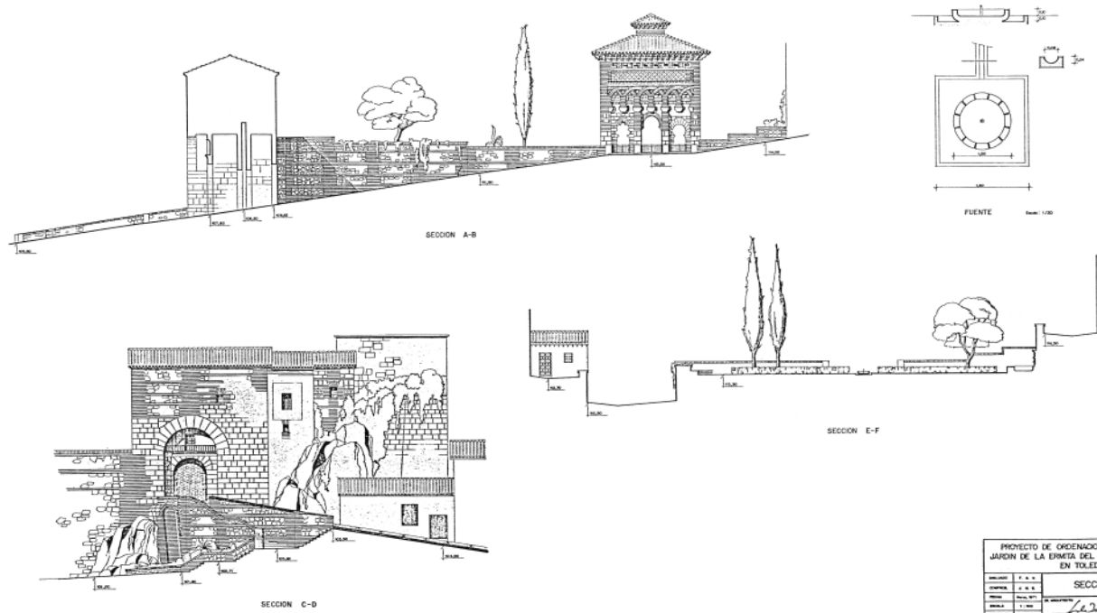
Site section and section terrace; Fountain: site section; basin plan and section
