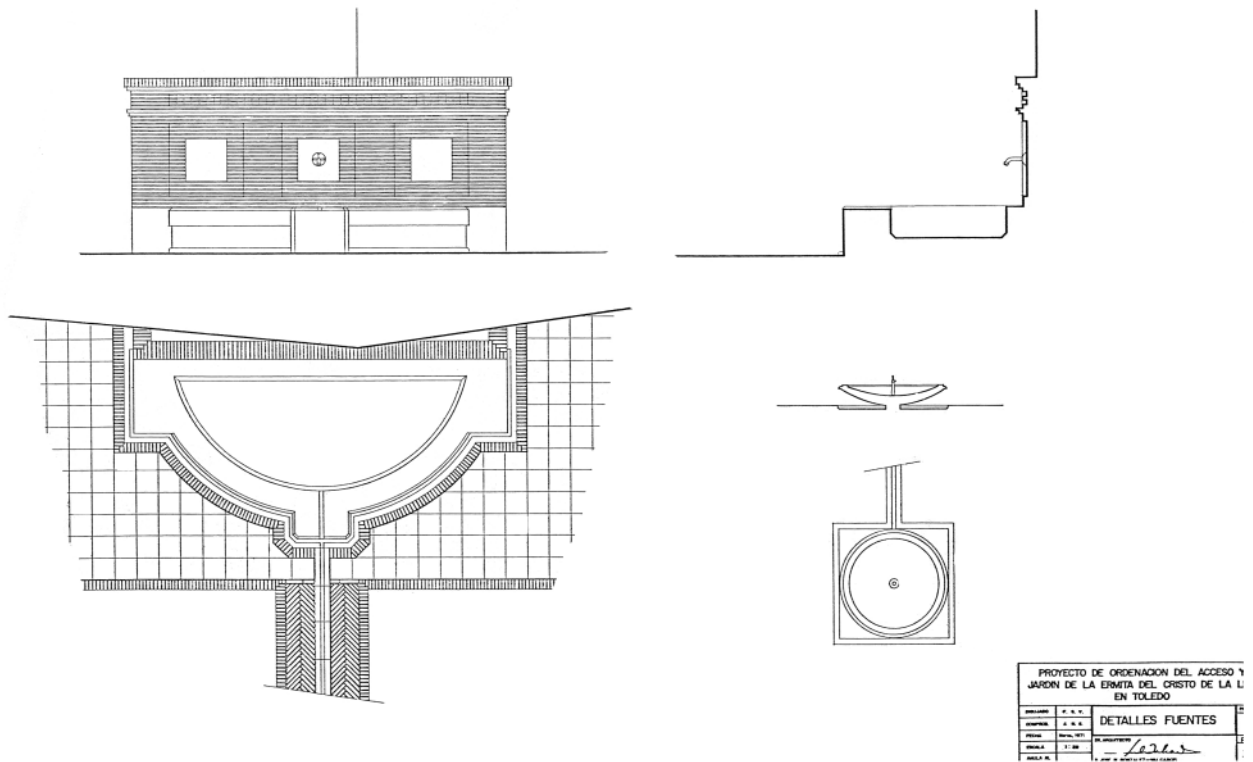
Fountain details of mosque terrace
