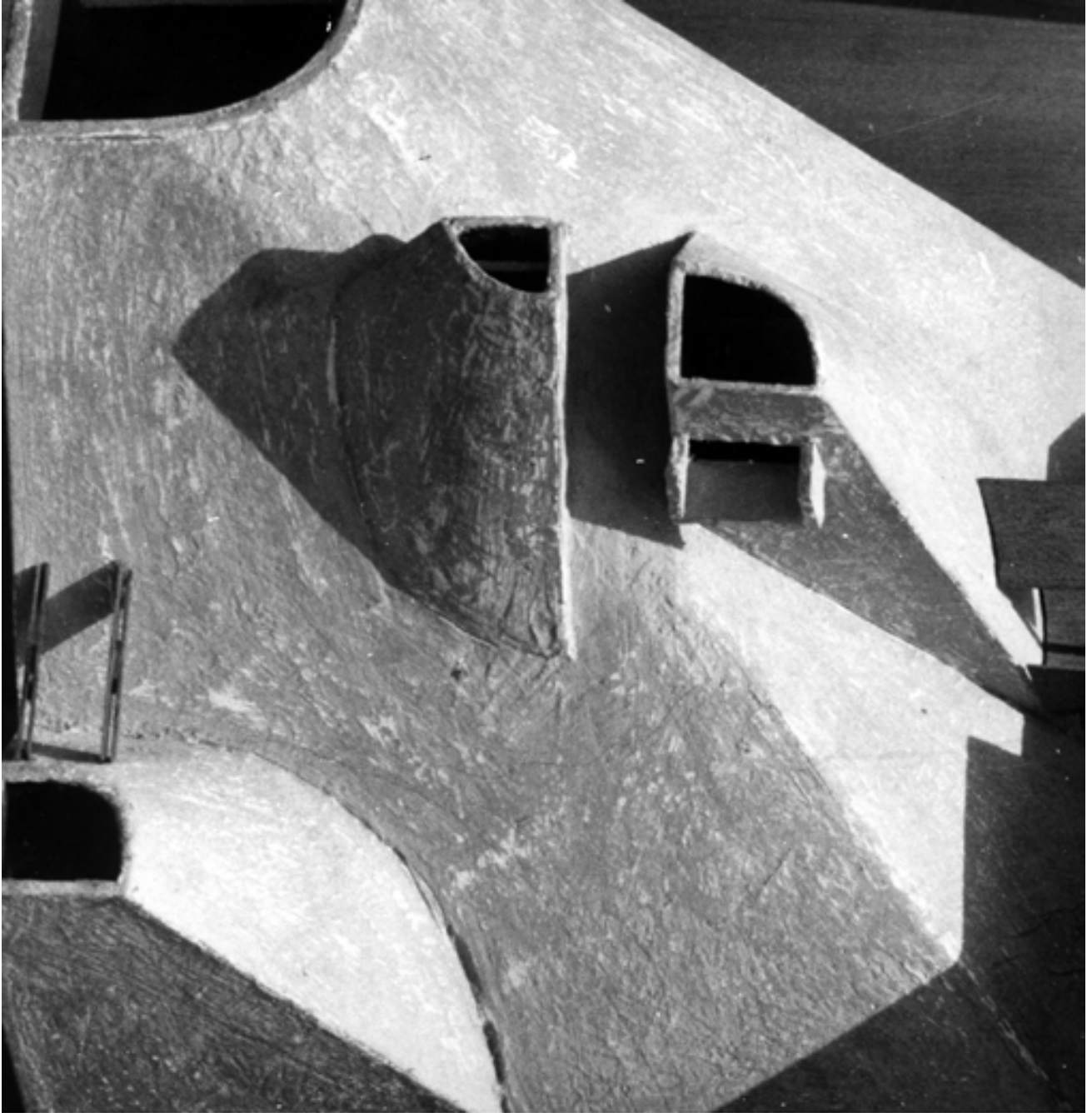
Concrete roof above prayer room and skylights
