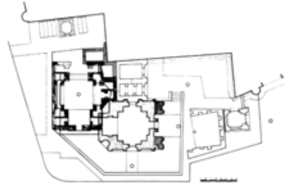
d) Uch Arkhona Mausoleum, project plan.
