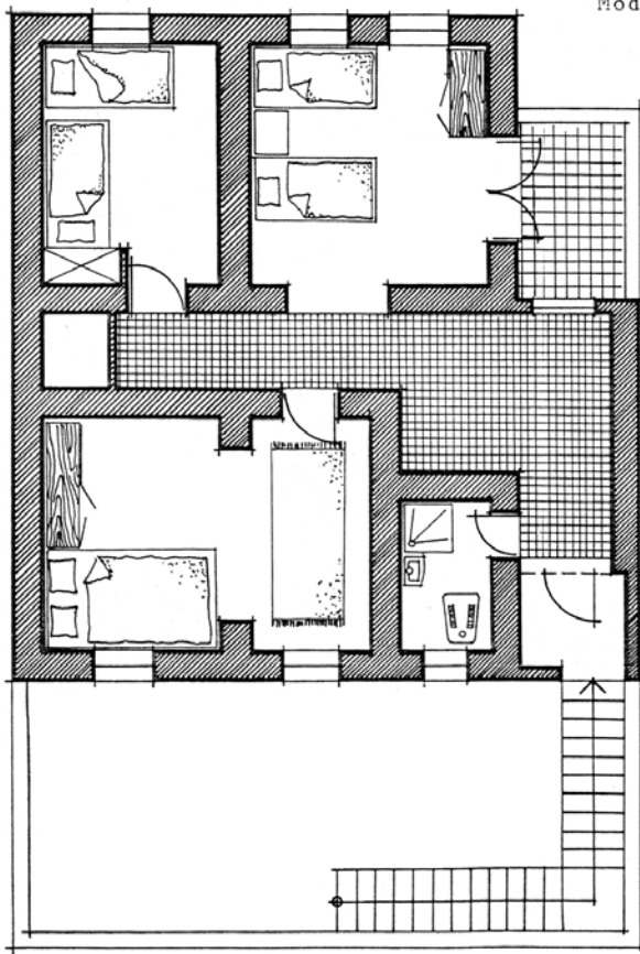
Groundplan - Groundfloor M 1:100
