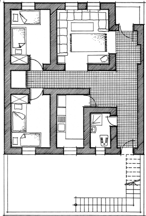
Groundplan - Upper floor M 1:100
