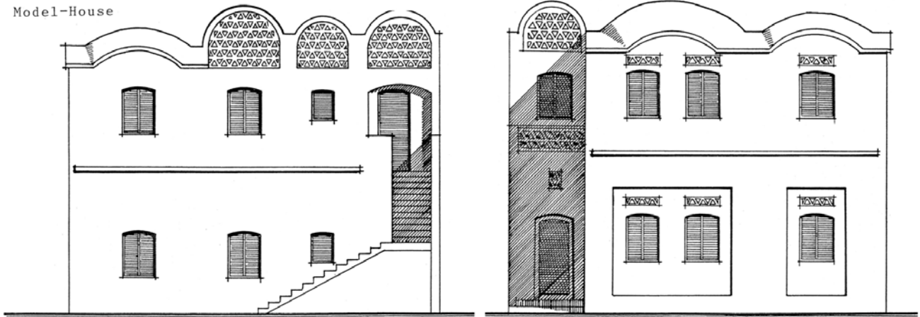
Facades M 1:100
